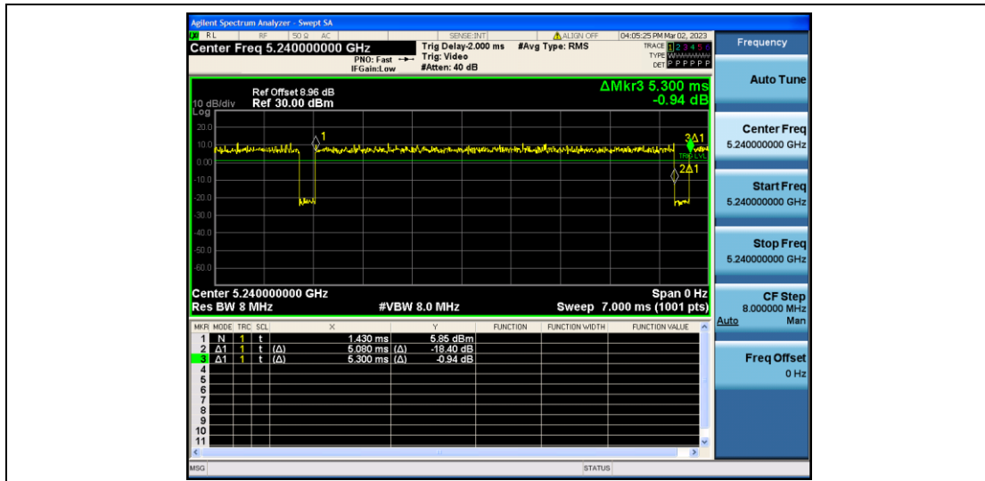
11N20SISO_Ant2_5240
