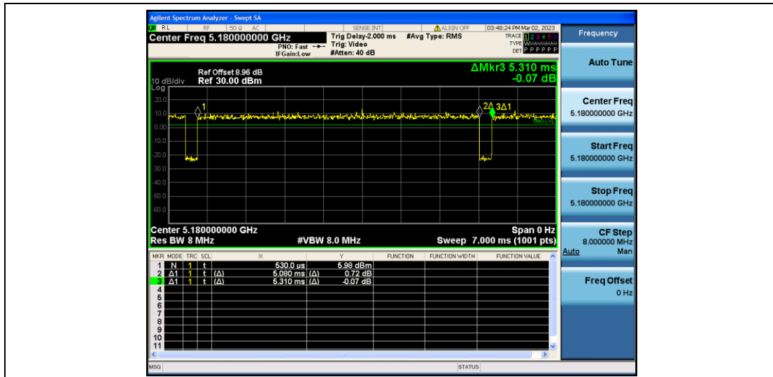
11N20SISO_Ant2_5180
