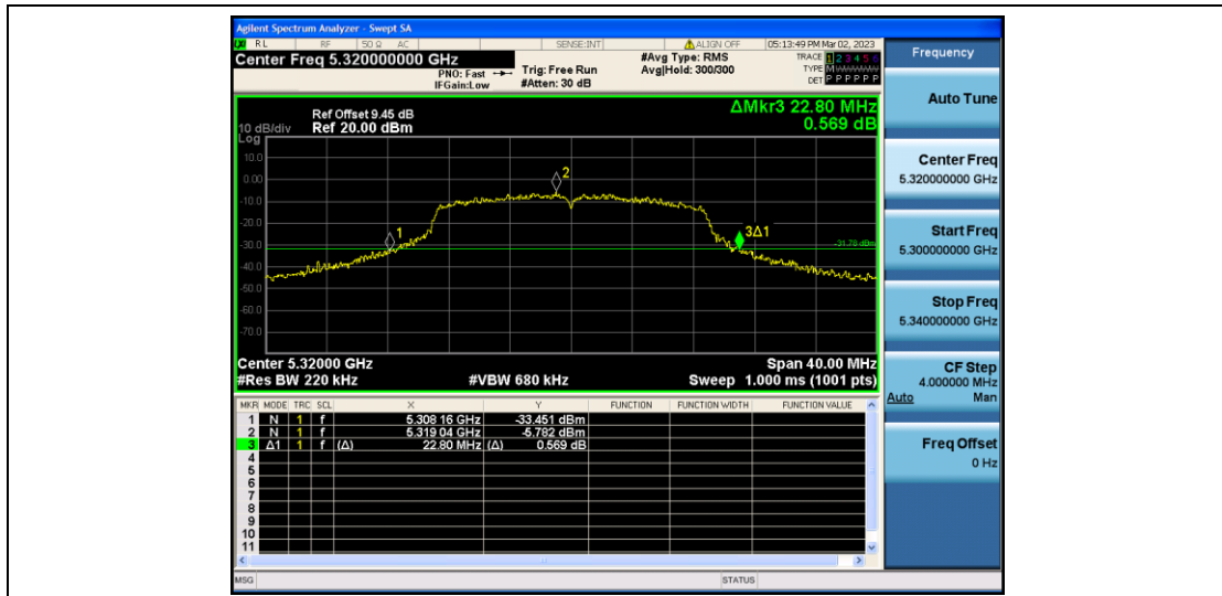
11N20SISO_Ant2_5320
