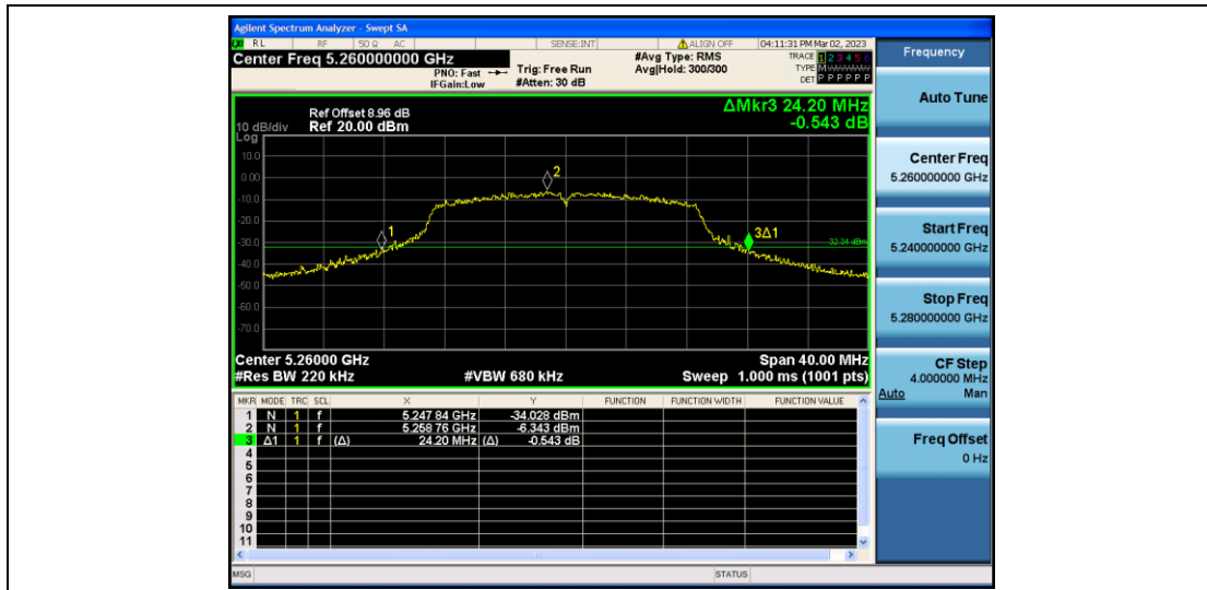
11N20SISO_Ant2_5260
