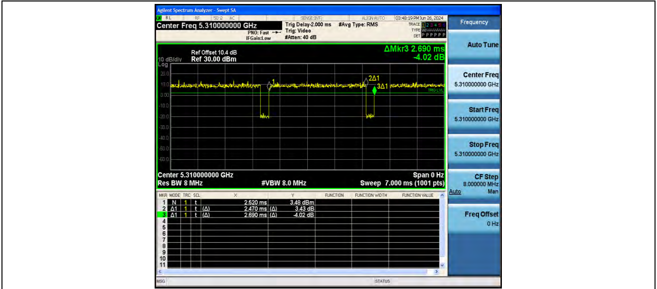
11N40SISO_Ant2_5310
