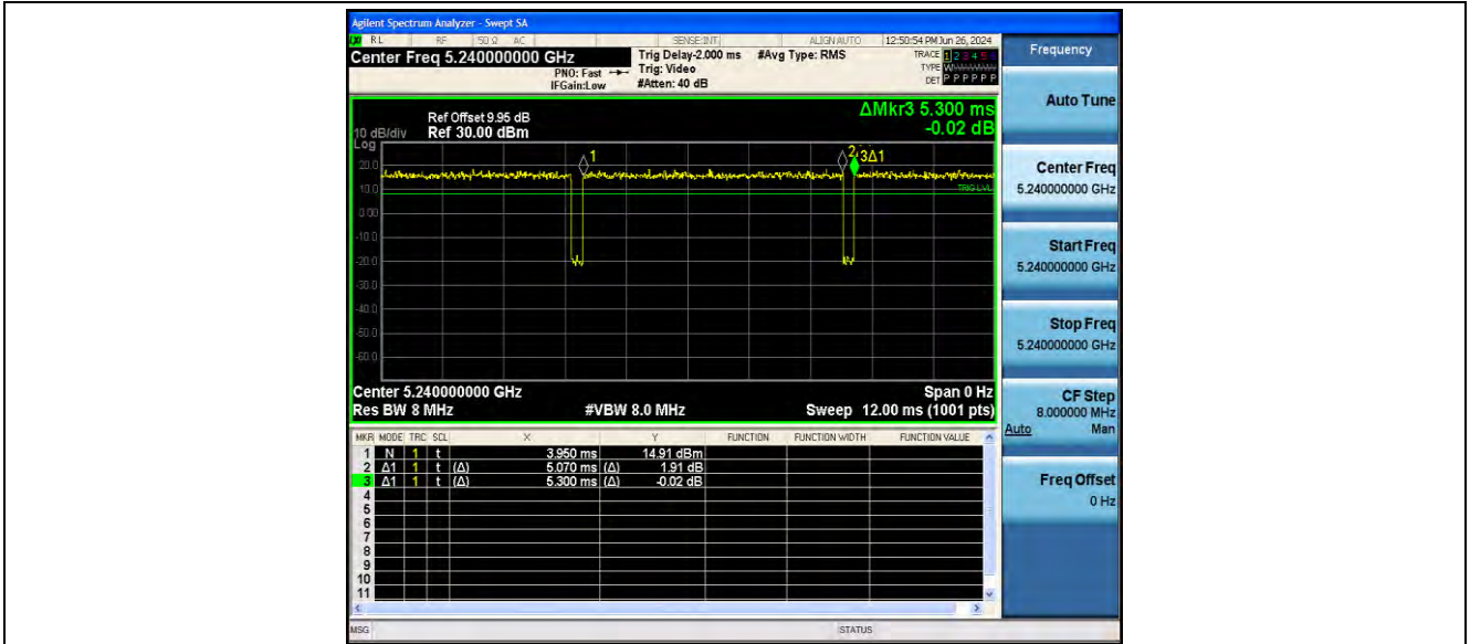
11N20SISO_Ant2_5240
