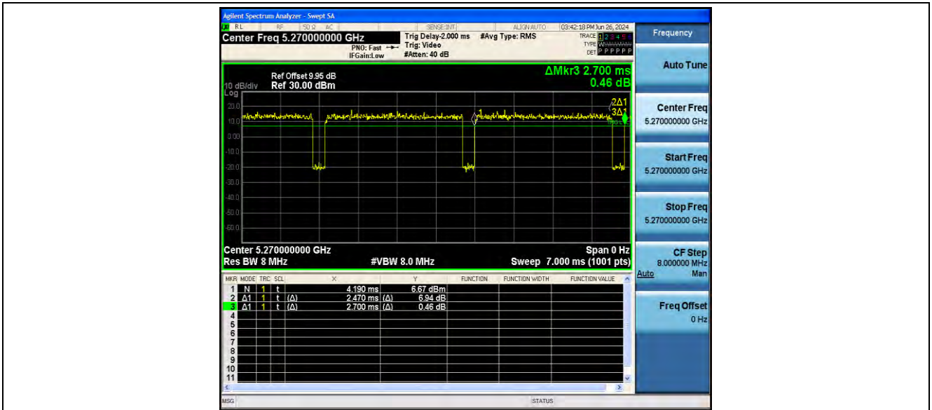
11N40SISO_Ant2_5270
