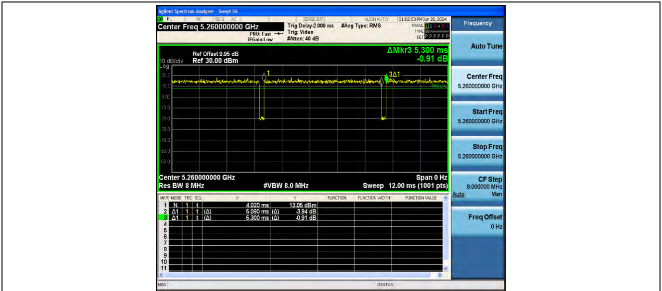
11N20SISO_Ant2_5260
