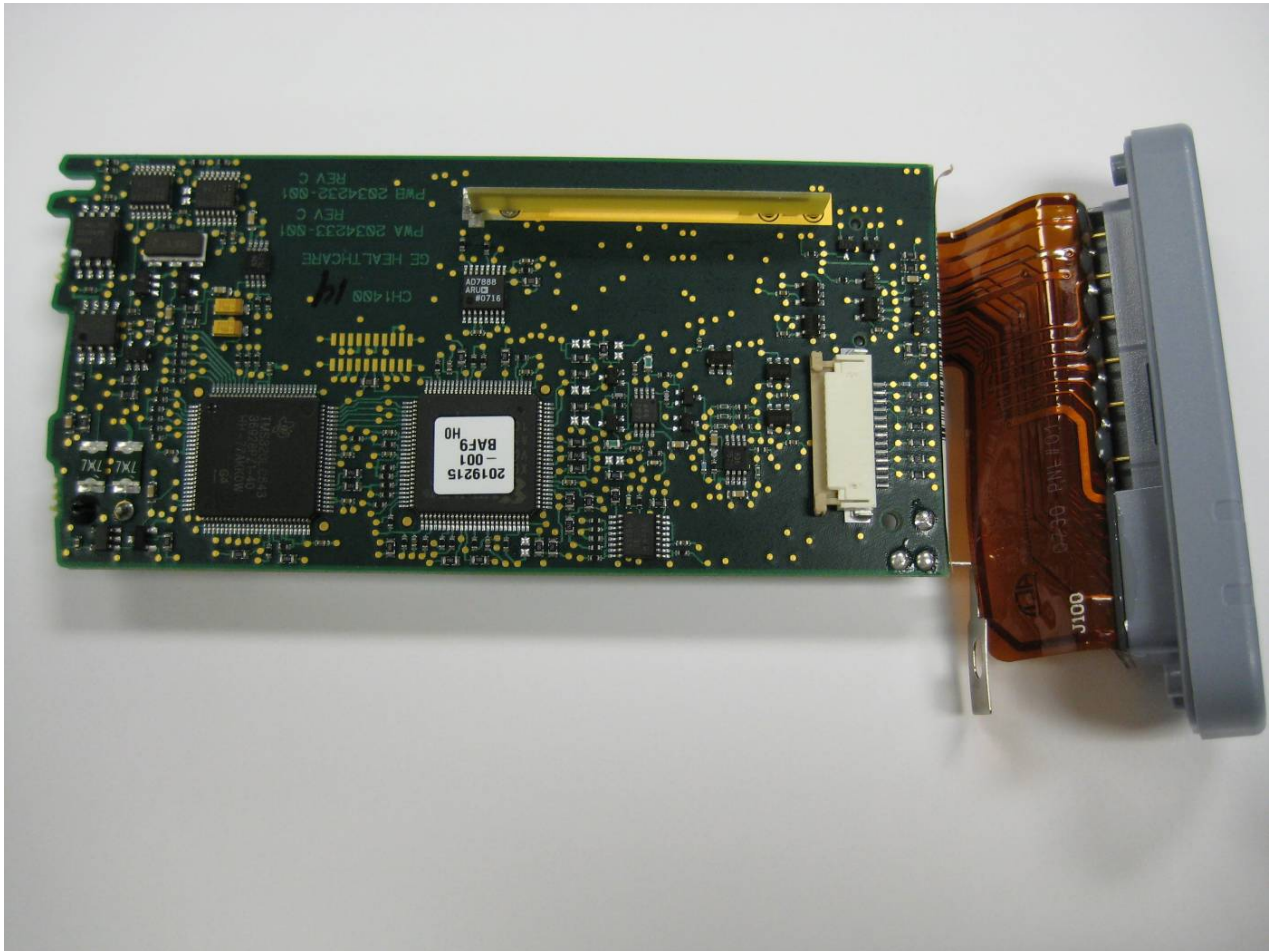
Back Side of Board – View #2
