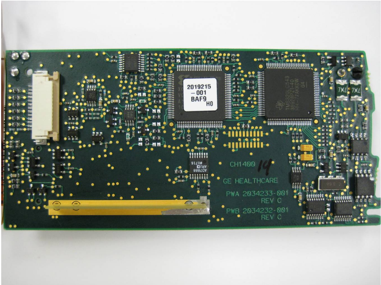
Back Side of Board – View #4
