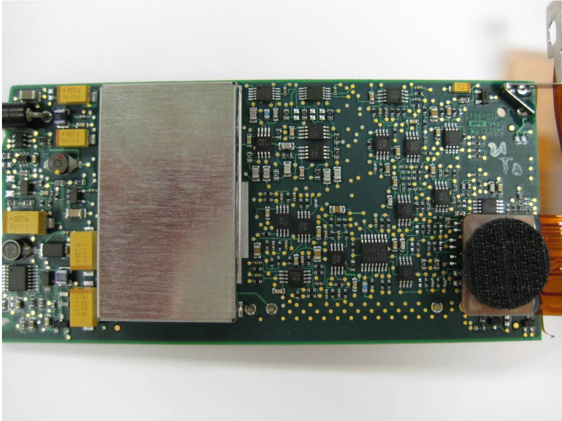
Open for Inspection, Close up – Shielded
