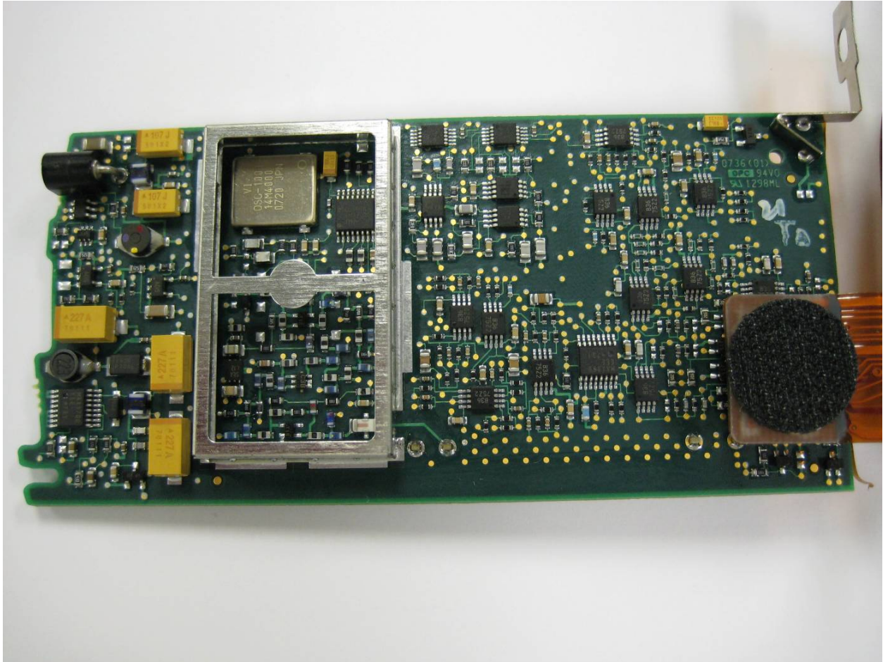
Close up – Shield Removed View #3
