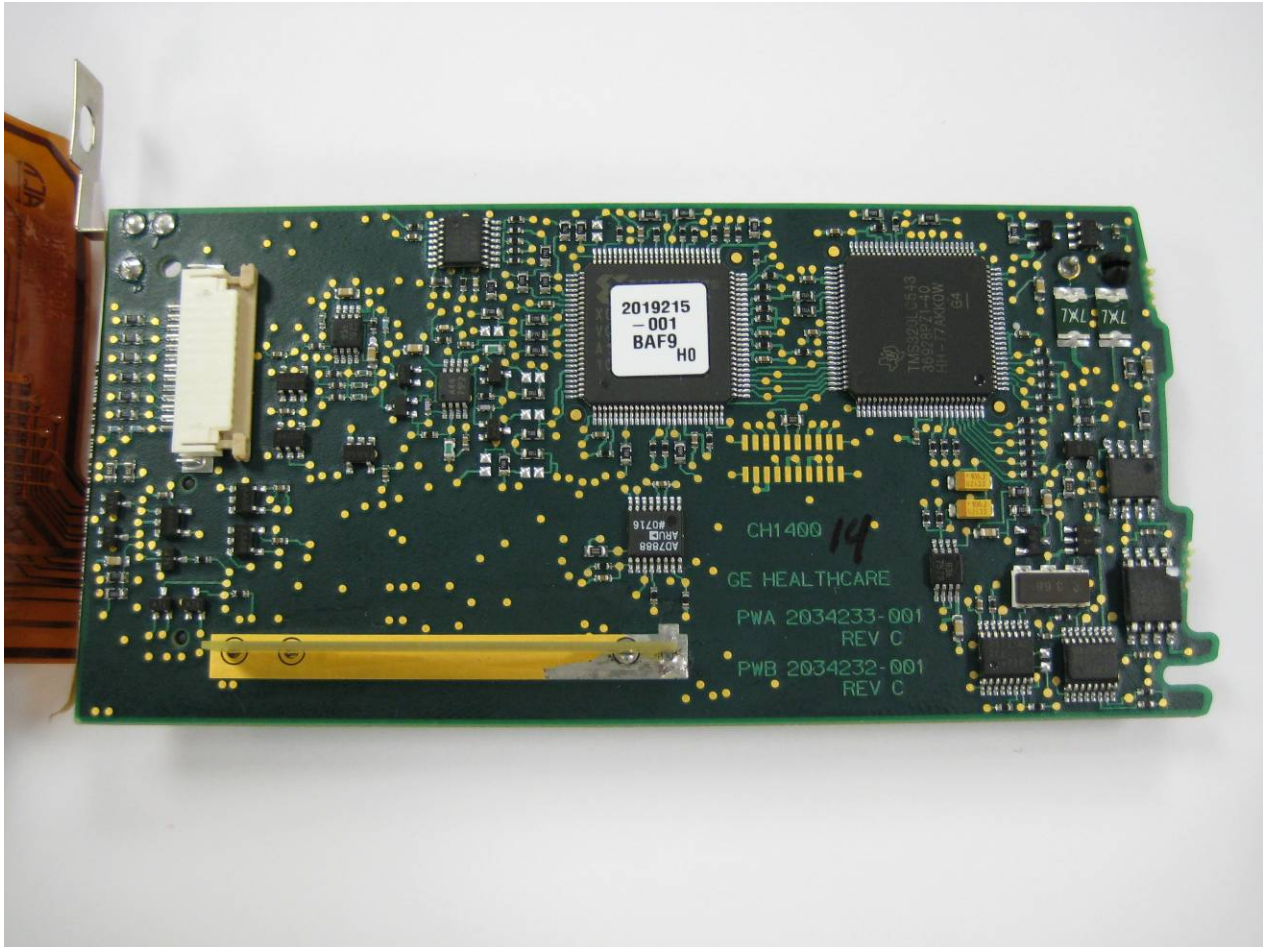
Back Side of Board – View #3
