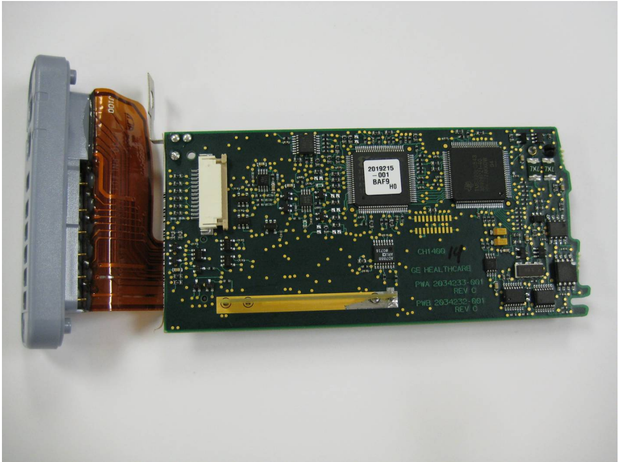
Back Side of Board – View #5
