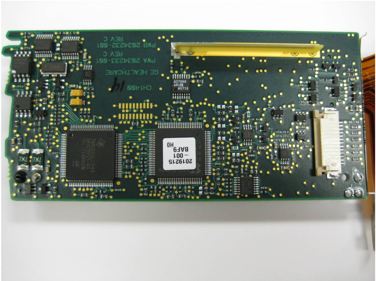
Back Side of Board – View #1
