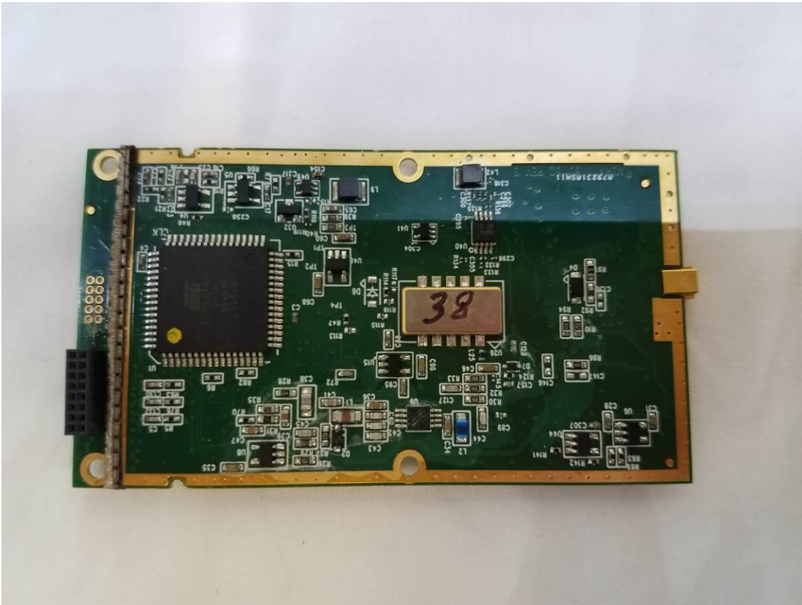
Figure 8. Inside of Radio Module – Bottom Side
