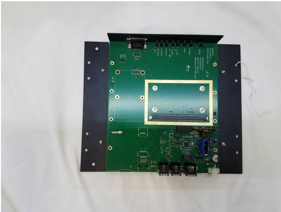
Figure 9. Unpopulated PCB Top Side
