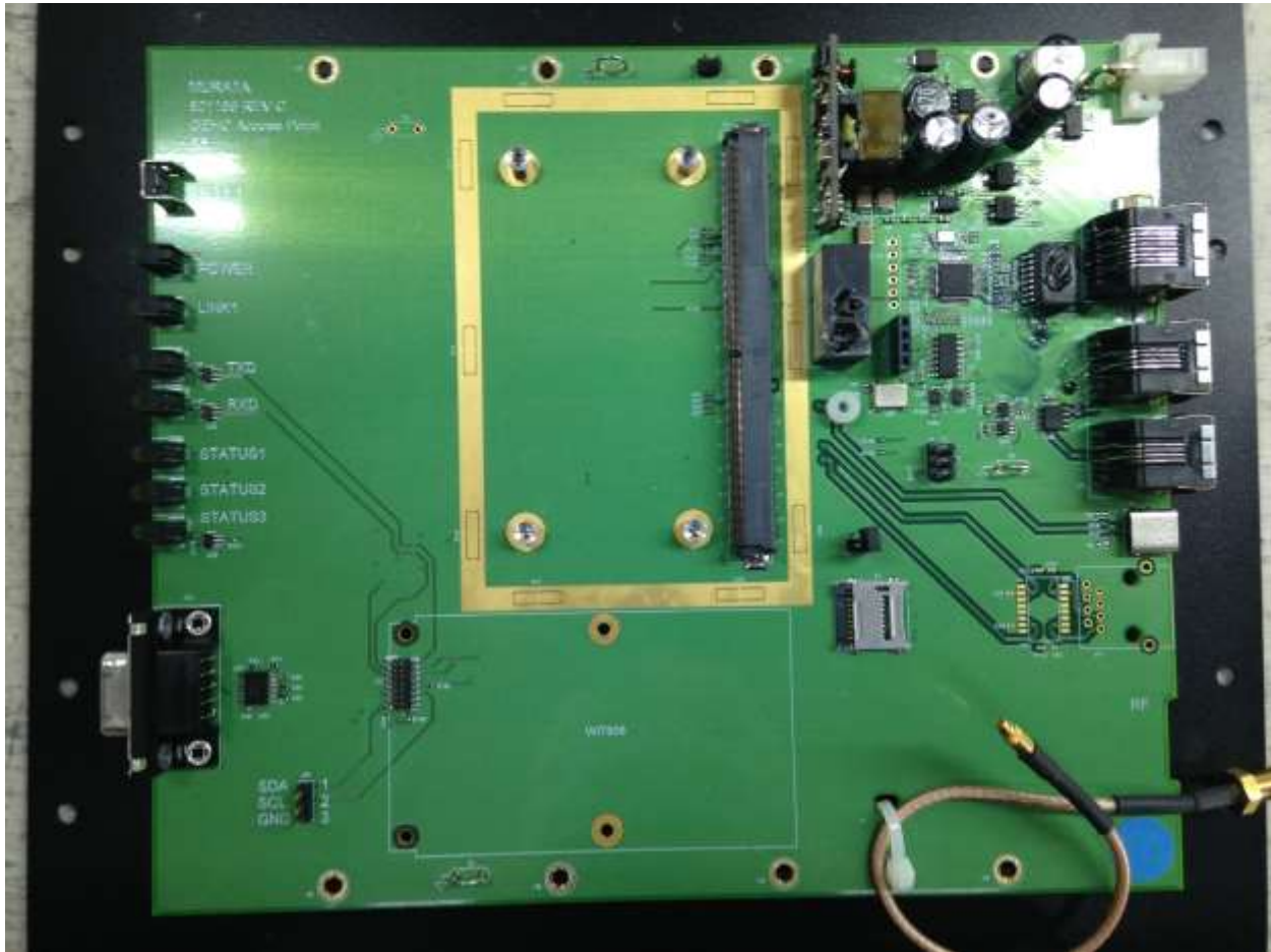
Figure 3. Modular PCBA Removed
