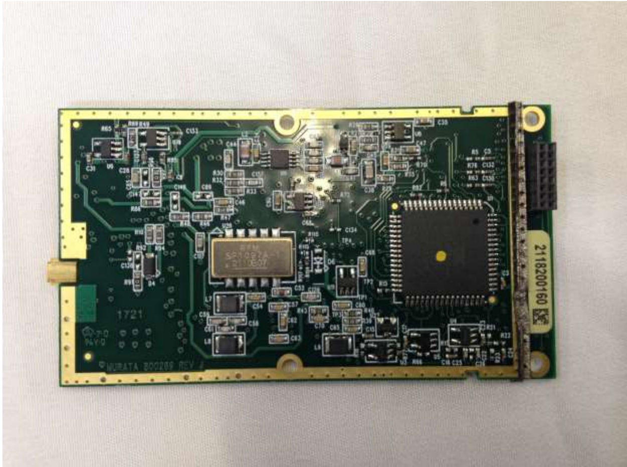
Figure 9. Module with Shield Removed, Bottom
