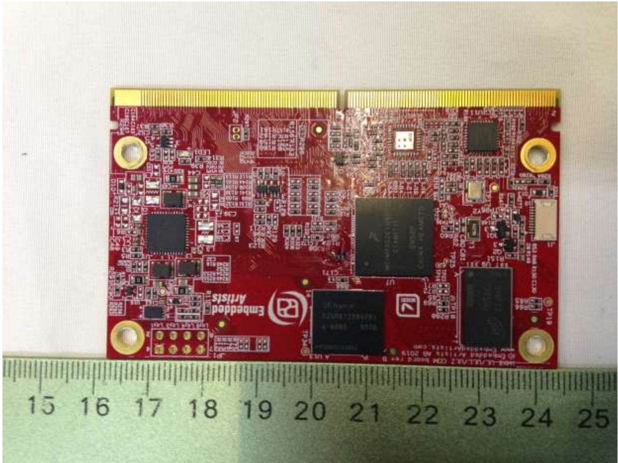
Figure 4. Embedded PCBA, Top
