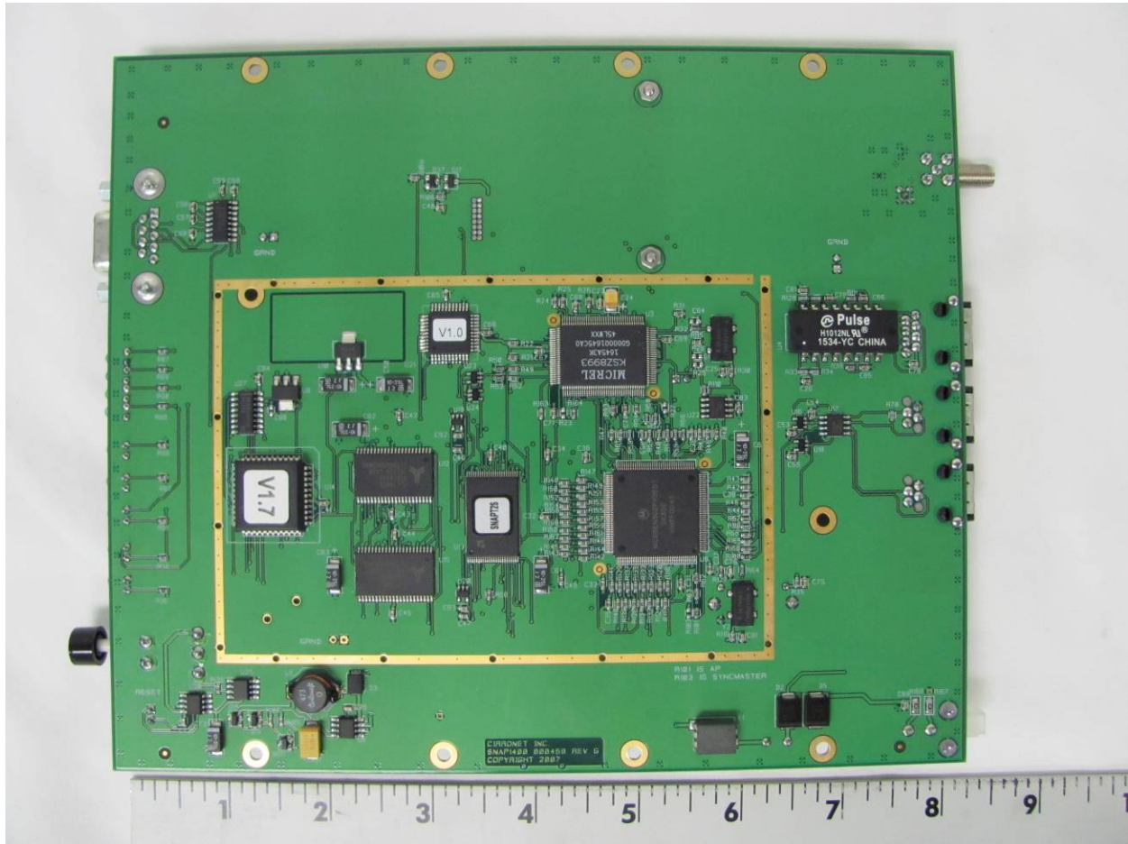
Figure 2. Main Board, Component Side
