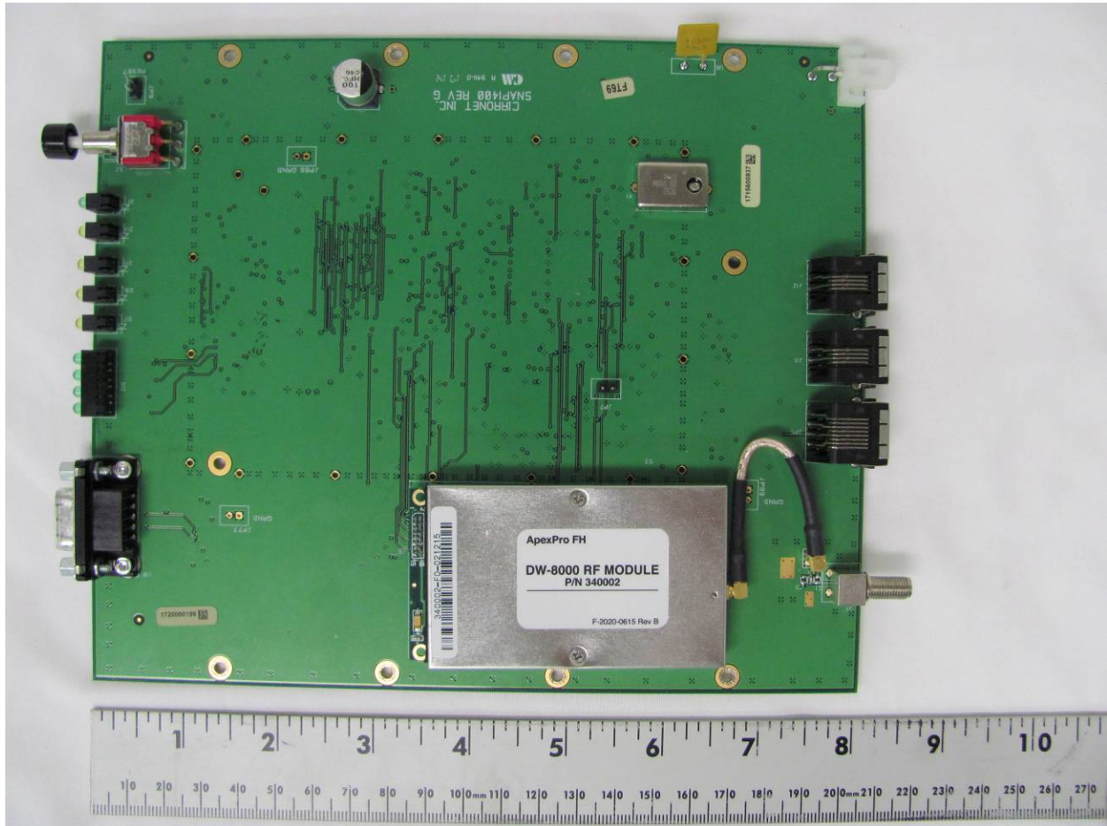
Figure 1. Main Board, Radio Side
