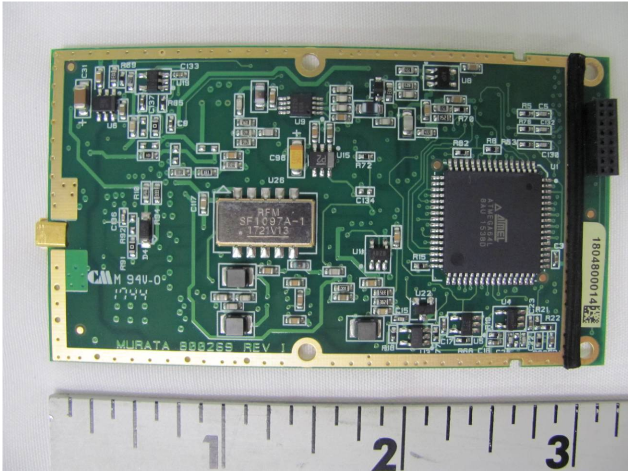
Figure 3. RF Module, Input Side
