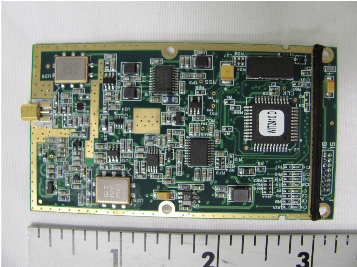
Figure 4. RF Module, Output Side
