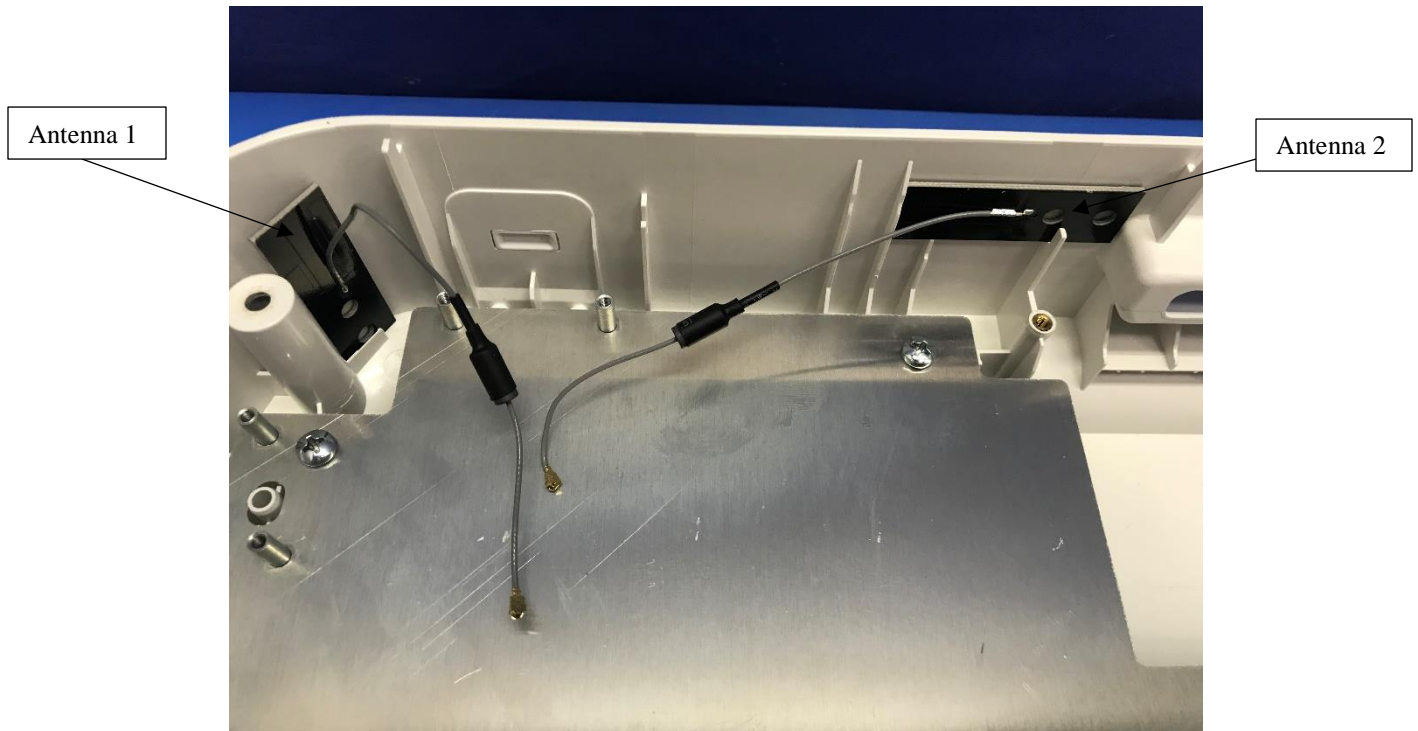
WiFi antenna
