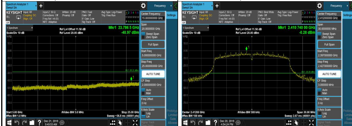
802.11n(HT20),2412MHz,Ant2,Plot 2,Band Edge
