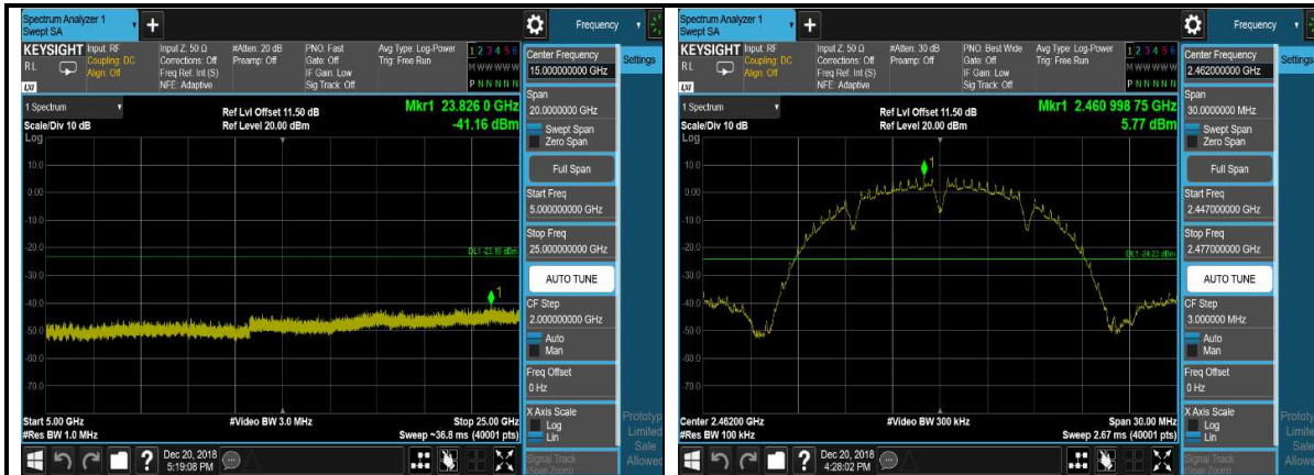
802.11b,2462MHz,Ant2,Plot 2,Band Edge
