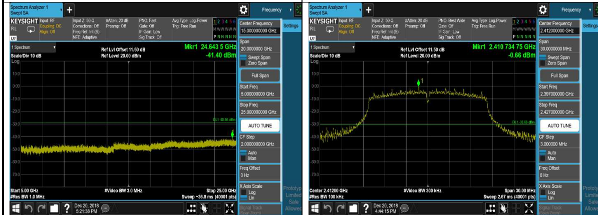
802.11g,2412MHz,Ant2,Plot 2,Band Edge
