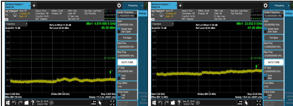
802.11n(HT20),2462MHz,Ant1,Plot 1,Reference Level
