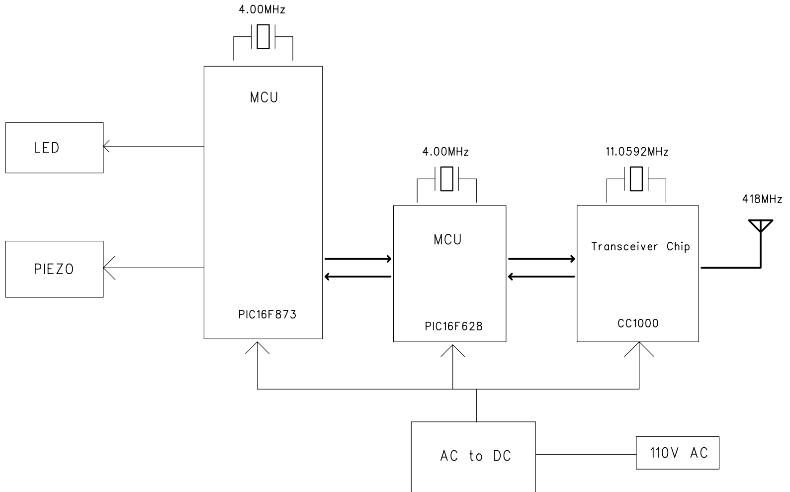
Figure 1. XWS350 Diagram block
