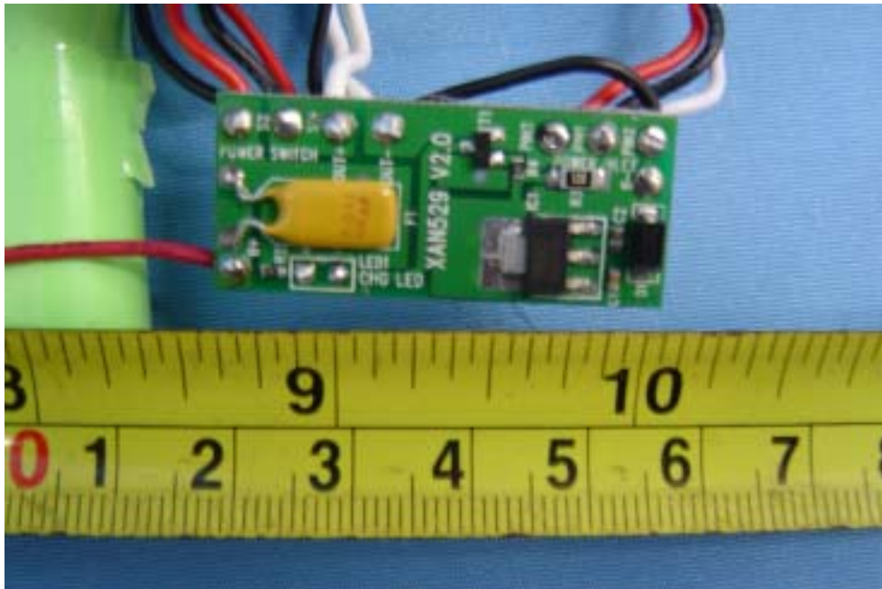
PCB - Component View(5)
