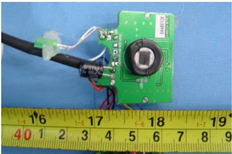
PCB - Solder View(4)
