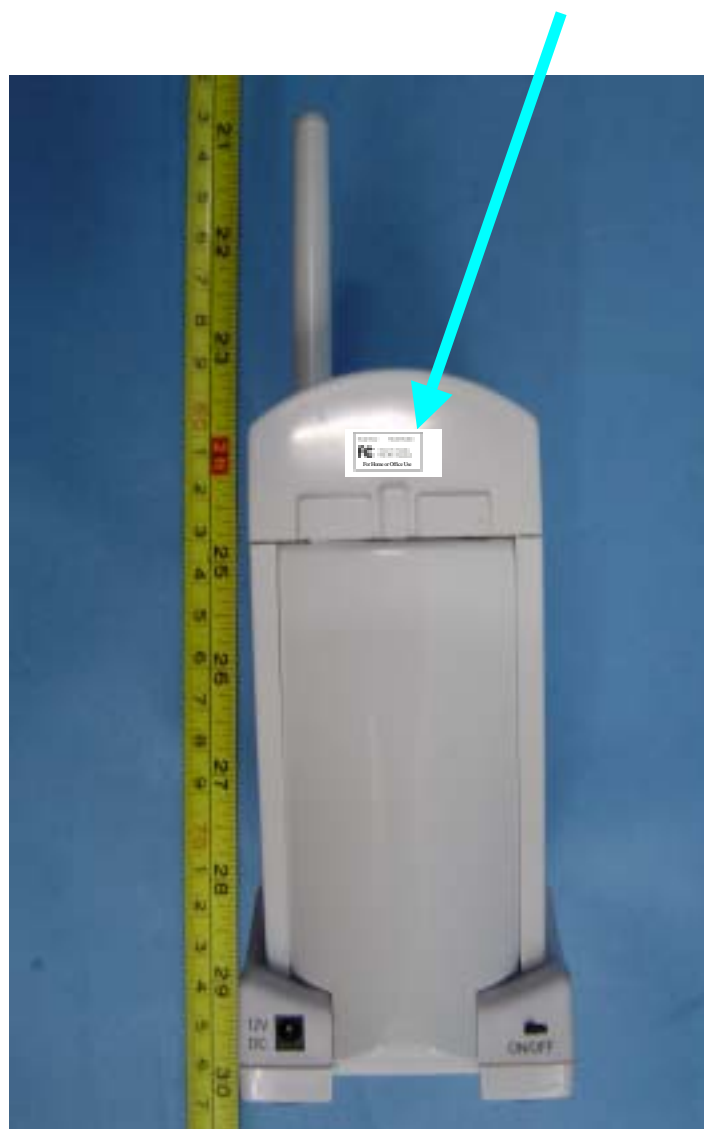
Proposed Label Location on EUT EUT Bottom View/proposed FCC Mark Location
