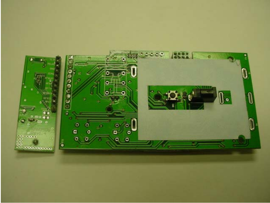
PCB Back
