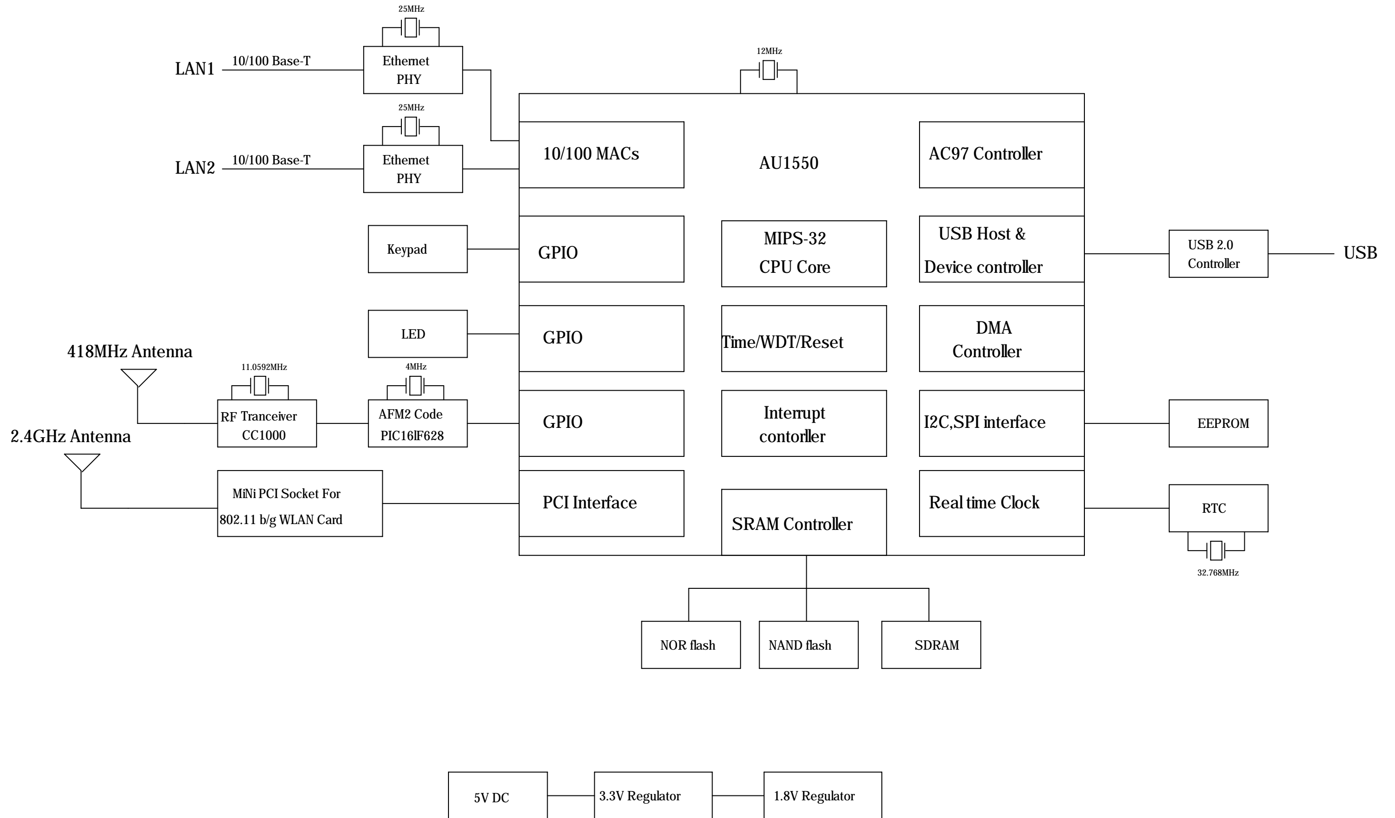
Figure 1. XG1000S-W Block Diagram
