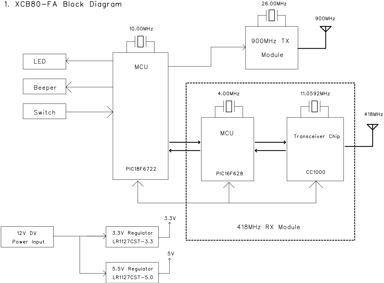
Figure 1. XCB80-FA Block Diagram
