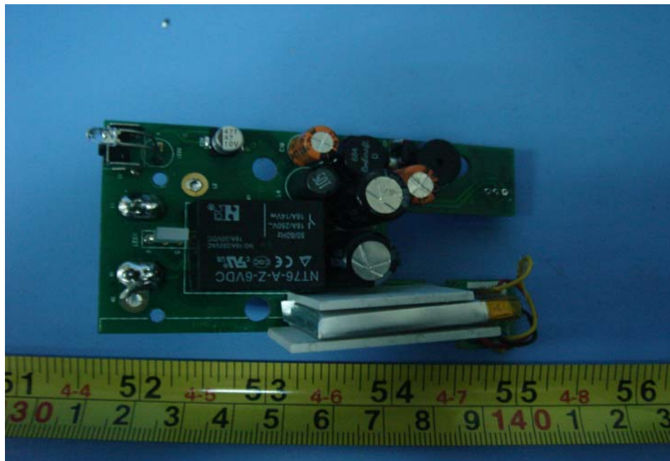
PCB-Back View(1)
