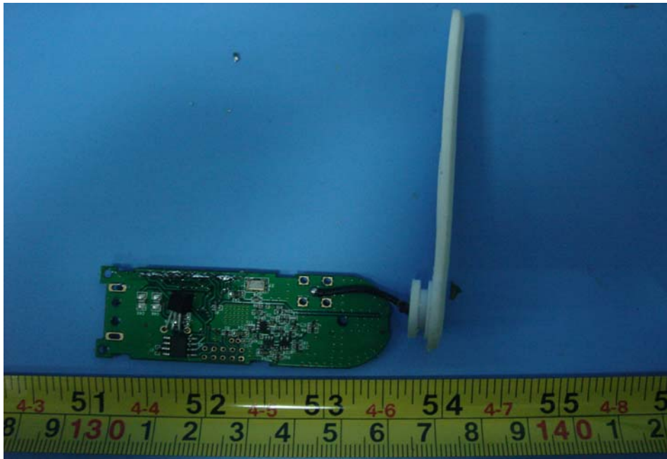
PCB-Back View(2)
