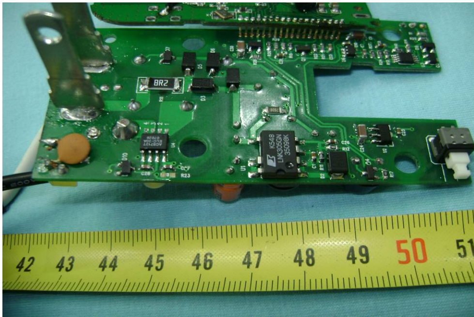
PCB-Back View(1)
