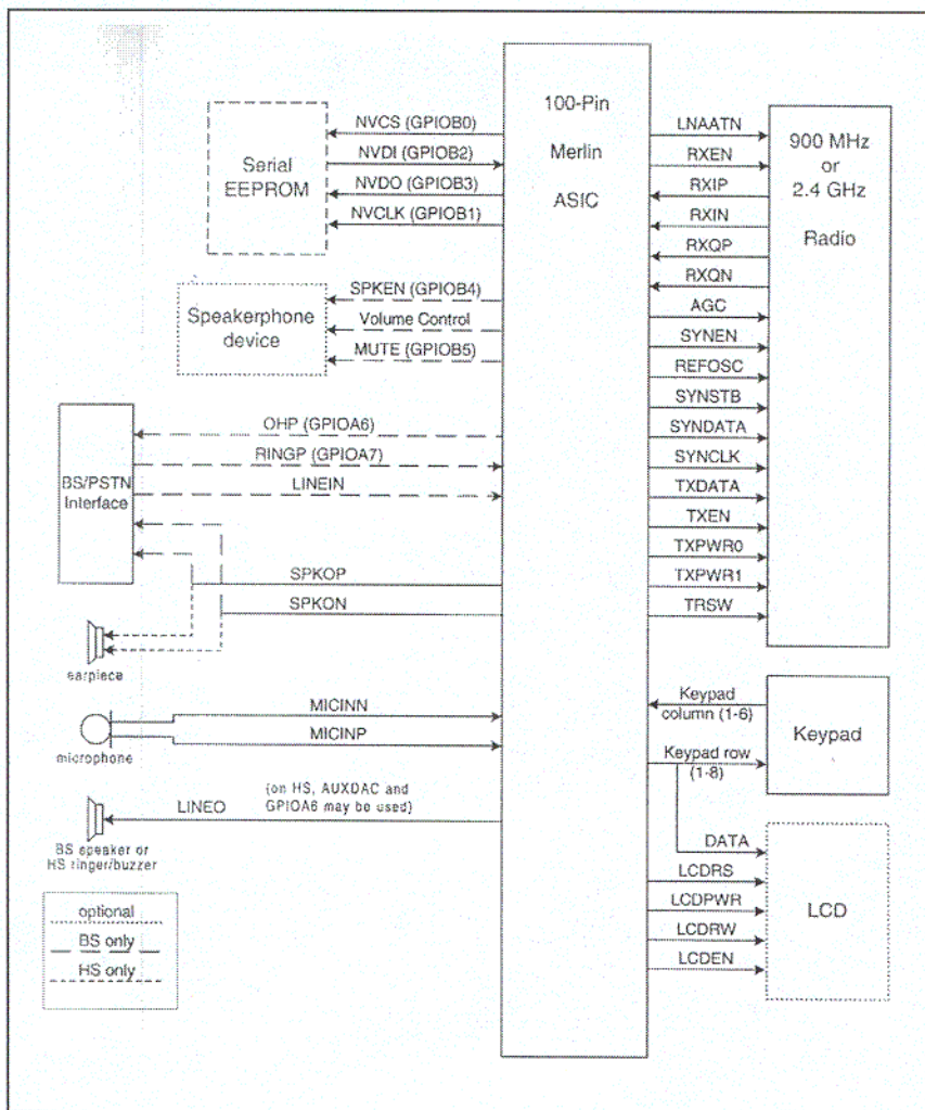
IBM3920 System Block Diagram
