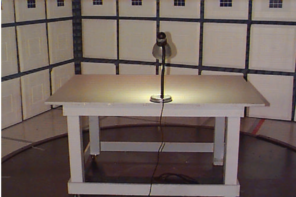
Maximized Radiated Emissions Test Set-up – Rear View
