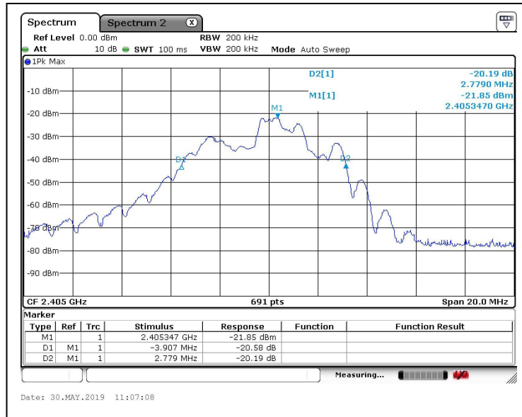
Channel: 2405MHz
