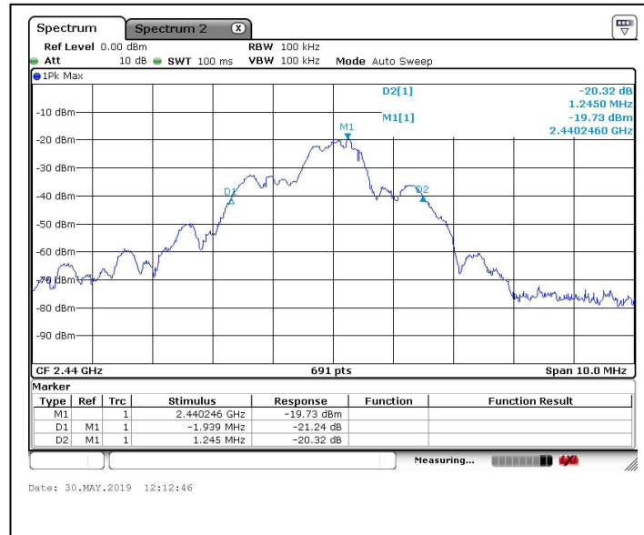
Channel: 2440MHz
