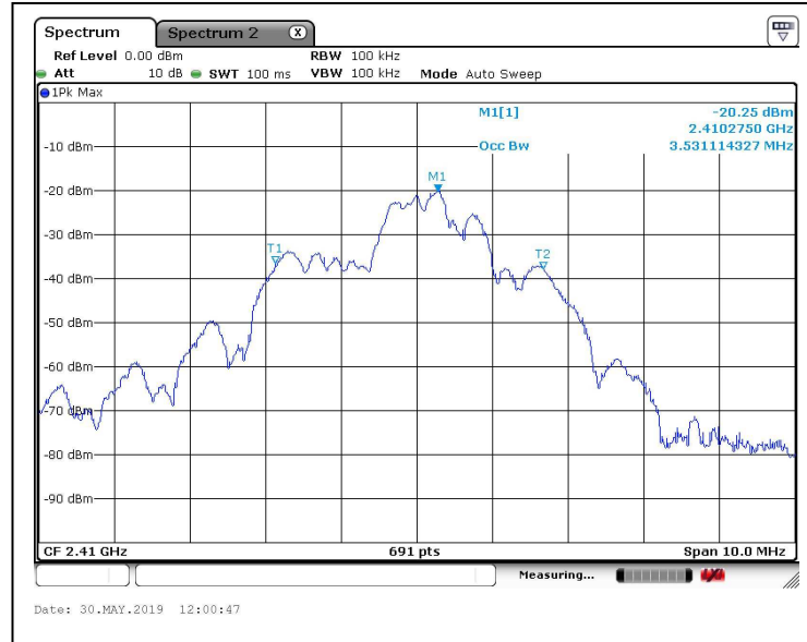
Channel: 2410MHz
