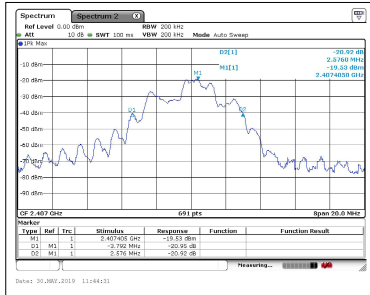
Channel: 2407MHz
