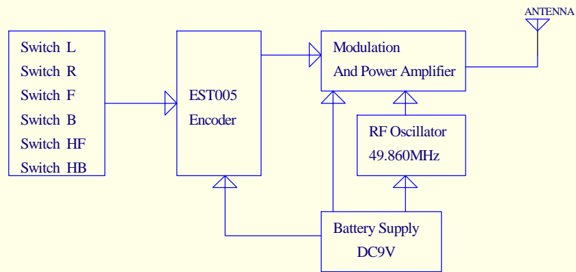
74147# Transmitter 49.860MHz Block Diagram
