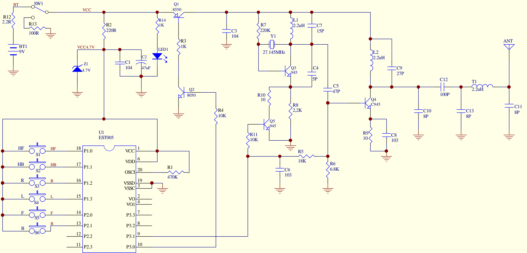
74146# Transmitter 27.145MHz Schematic
