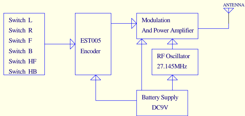
74146# Transmitter 27.145MHz Block Diagram
