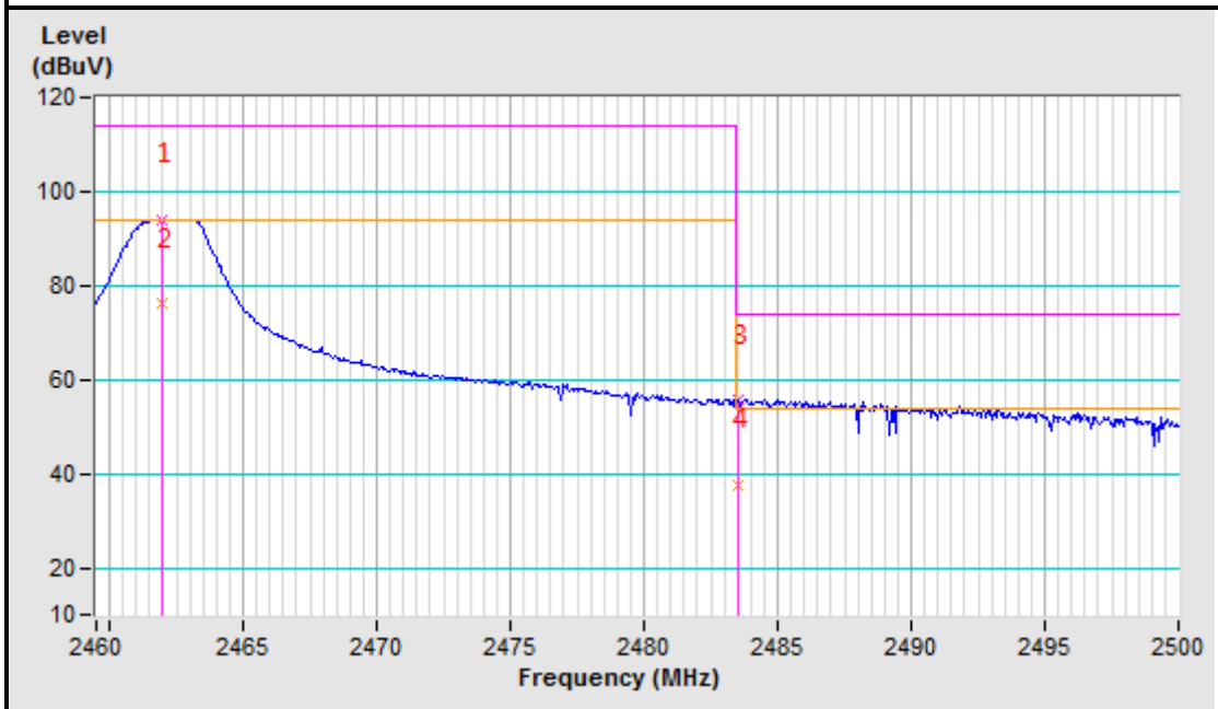
2462MHz Vertical
