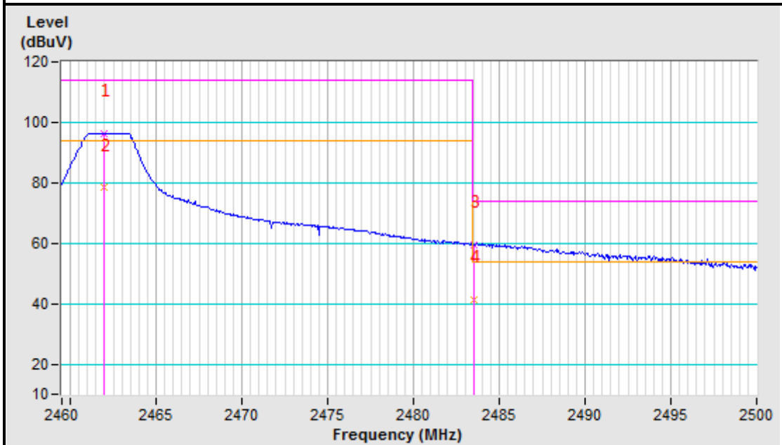
2462MHz Vertical
