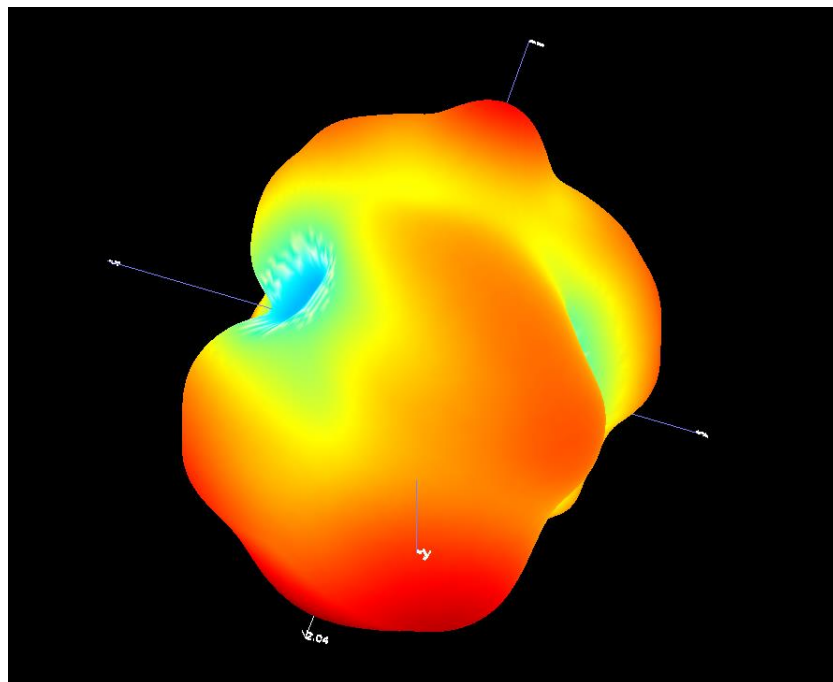
B1.2 3D Pattern for 2442MHz
