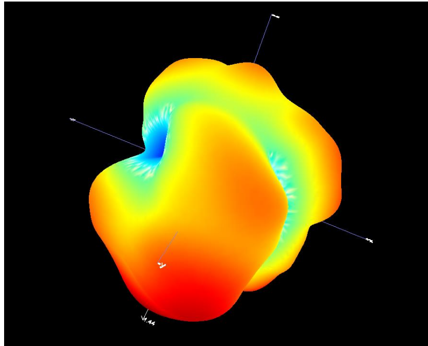
B1.1 3D Pattern for 2405MHz
