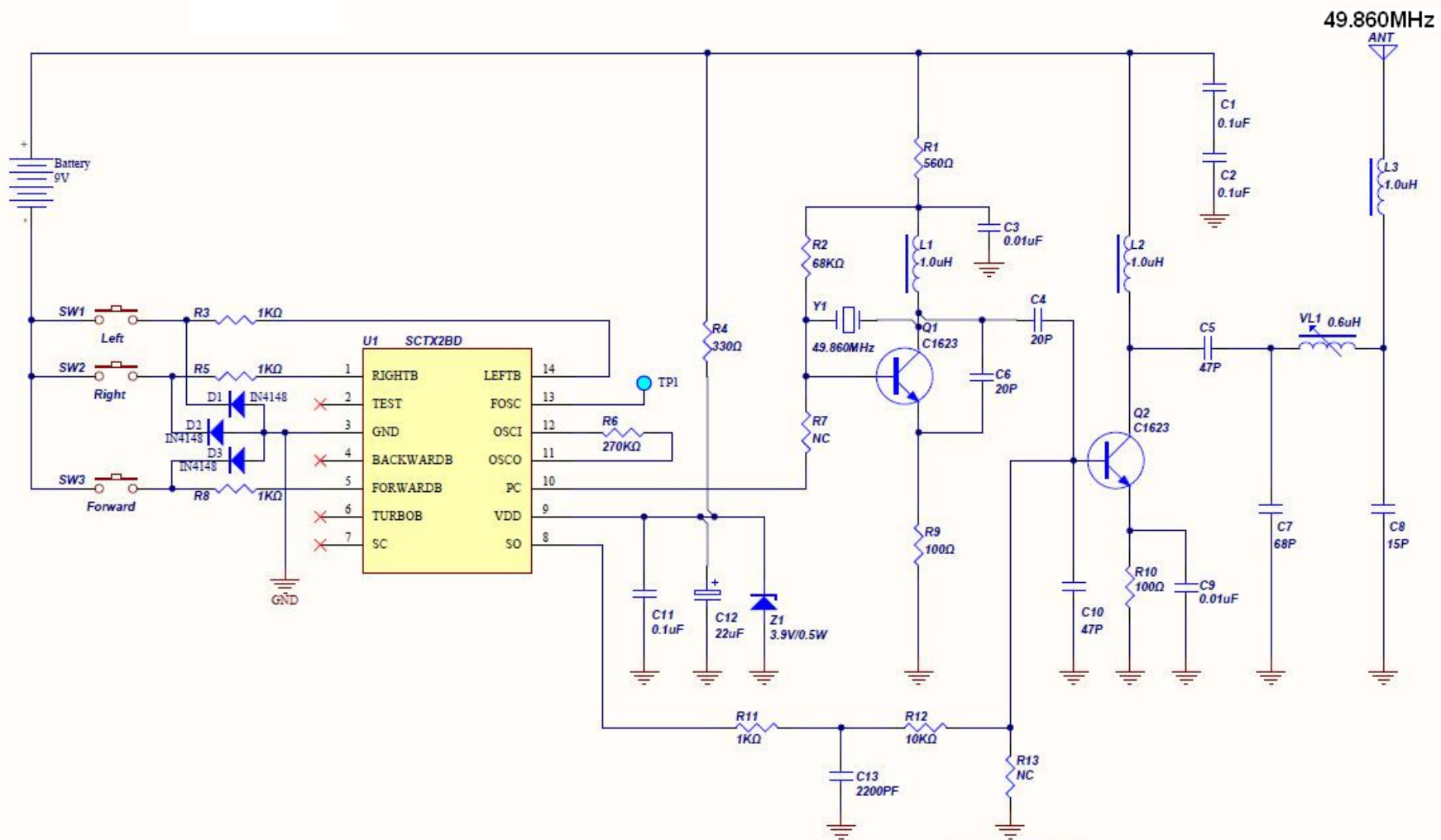
Schematic of Tx FCC ID: OTA74045T49 49.680MHz
