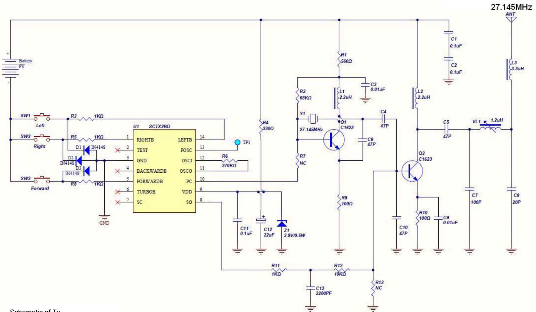
Schematic of Tx FCC ID: OTA74045T27 27.145MHz
