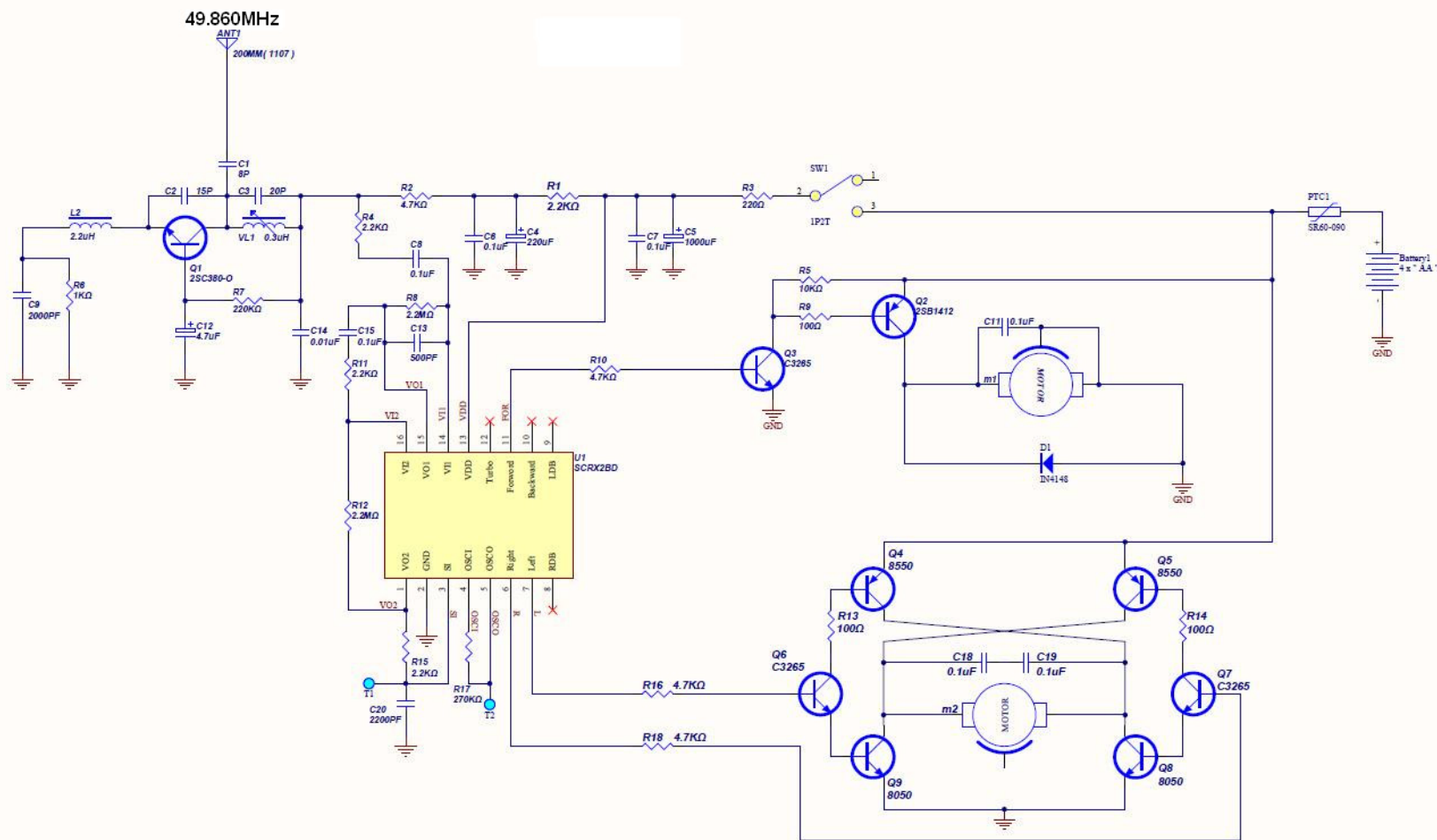
Schematic of Rx FCC ID: OTA74045R49 49.860MHz
