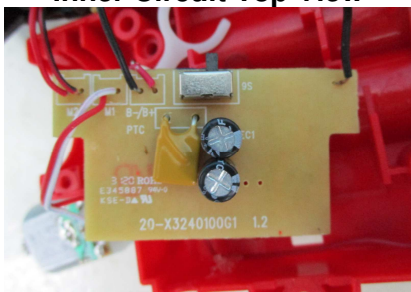
Inner Circuit Top View
