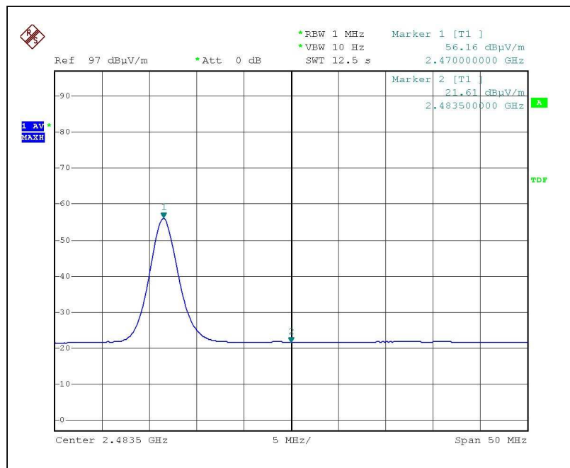
Bandwidth 4 (2.4835GHz Edge with Average Detector)
