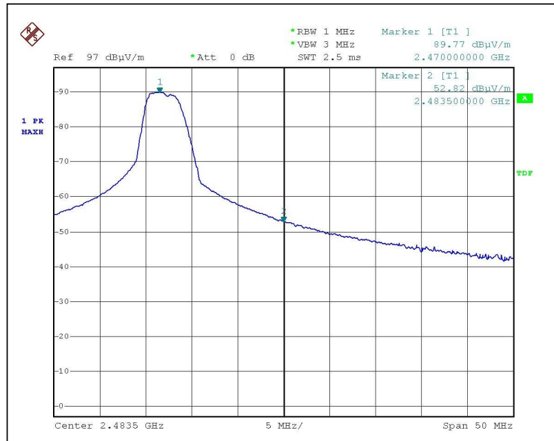
Bandwidth 3 (2.4835GHz Edge with Peak Detector)
