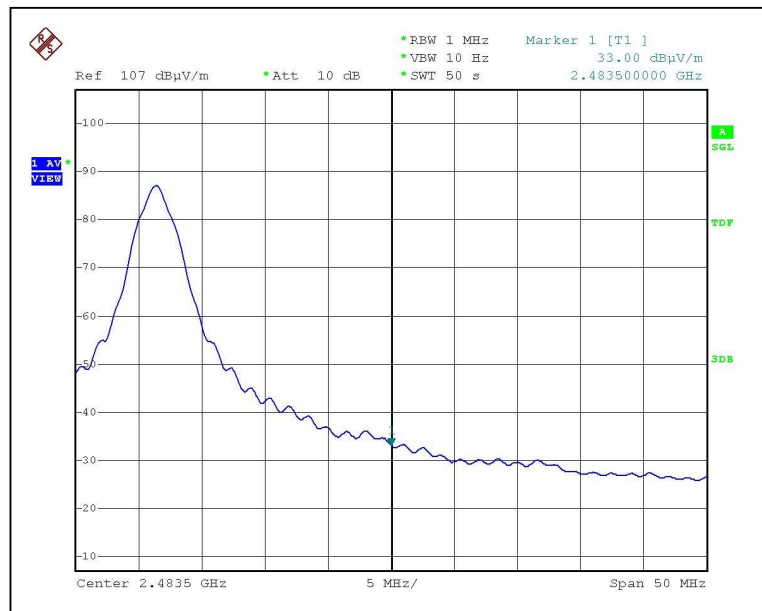
Band Edge 4 (2.4835GHz Edge with Average Detector)
