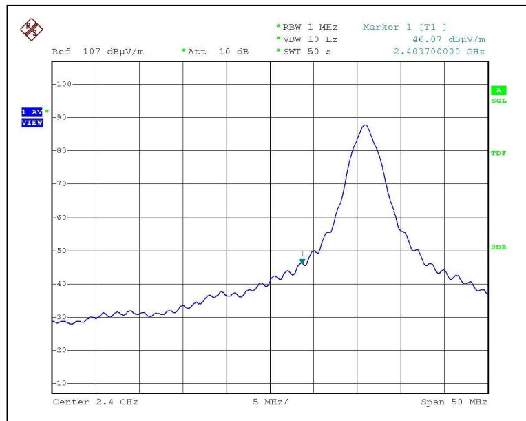
Band Edge 2 (2.4GHz Edge with Average Detector)
