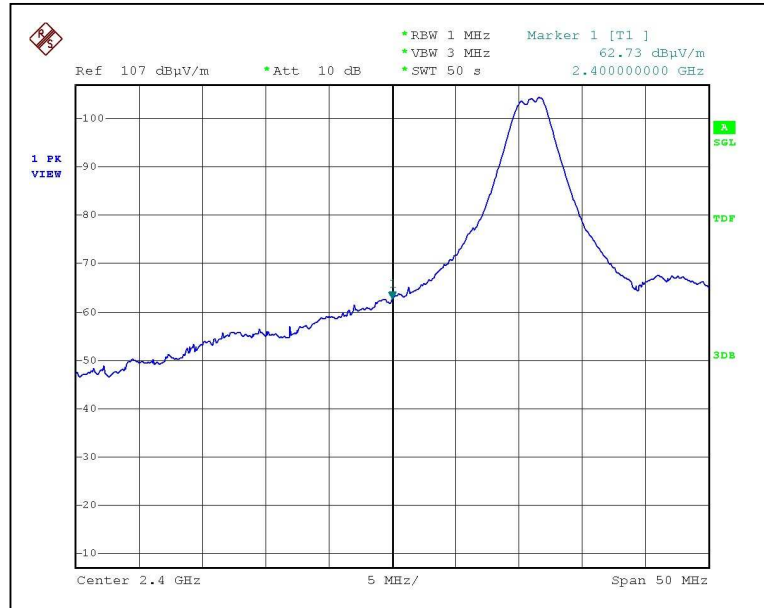
Band Edge 1 (2.4GHz Edge with Peak Detector)
