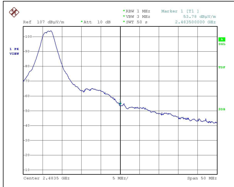
Band Edge 3 (2.4835GHz Edge with Peak Detector)
