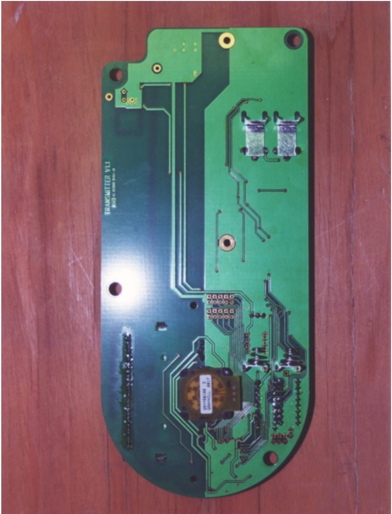
SOLDER SIDE OF BOARD (TRANSMITTER)
