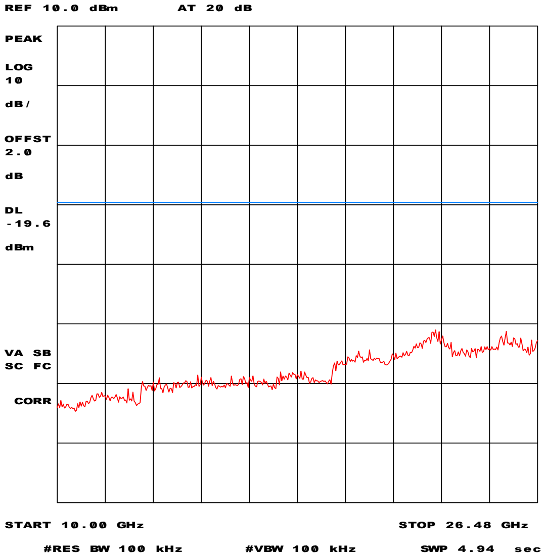
Plot 24 - Conducted emission outside restricted band (OFDM mode).
