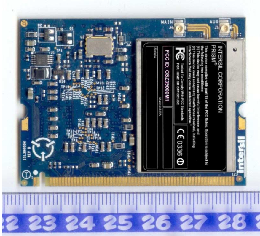
ISL3900M PCB front with shield
