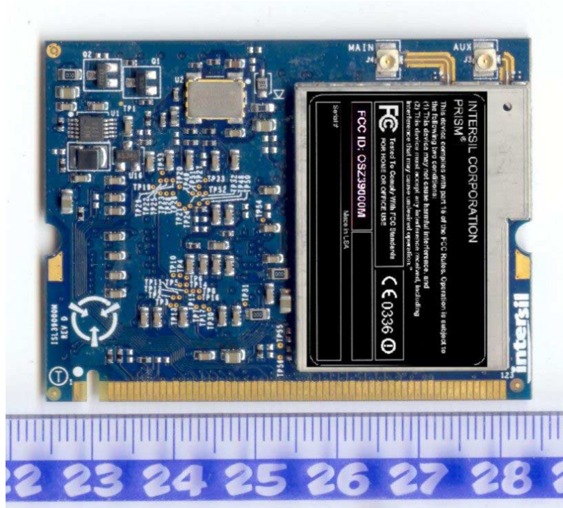
ISL3900M PCB front with shield
