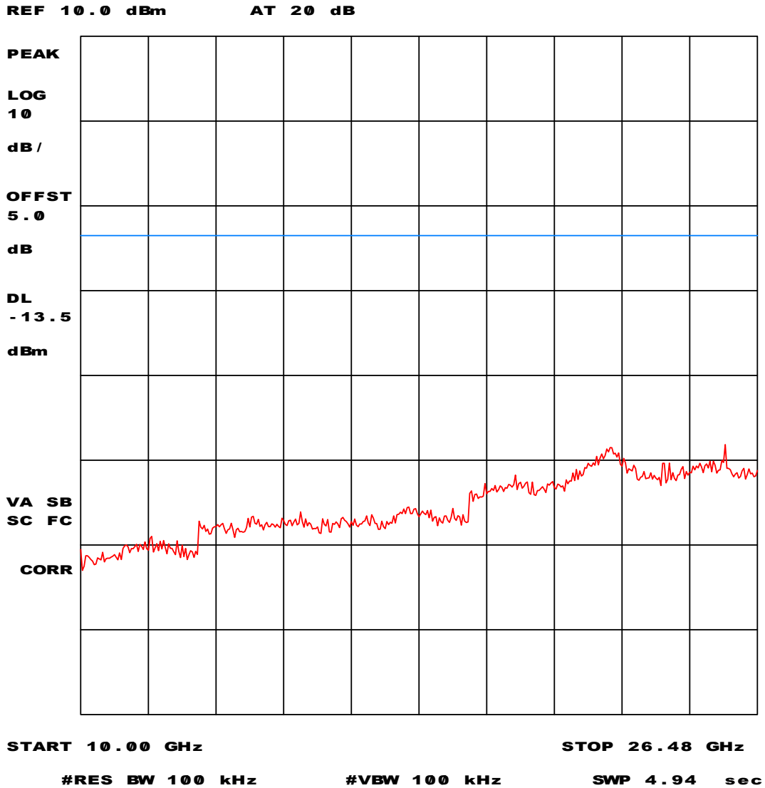
Plot 12 - Conducted emission outside restricted band.
