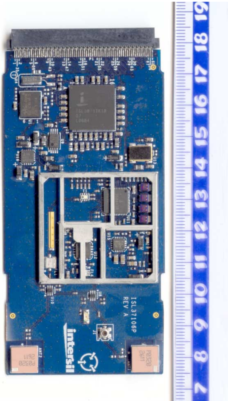
ISL37106P PCB front without shield
