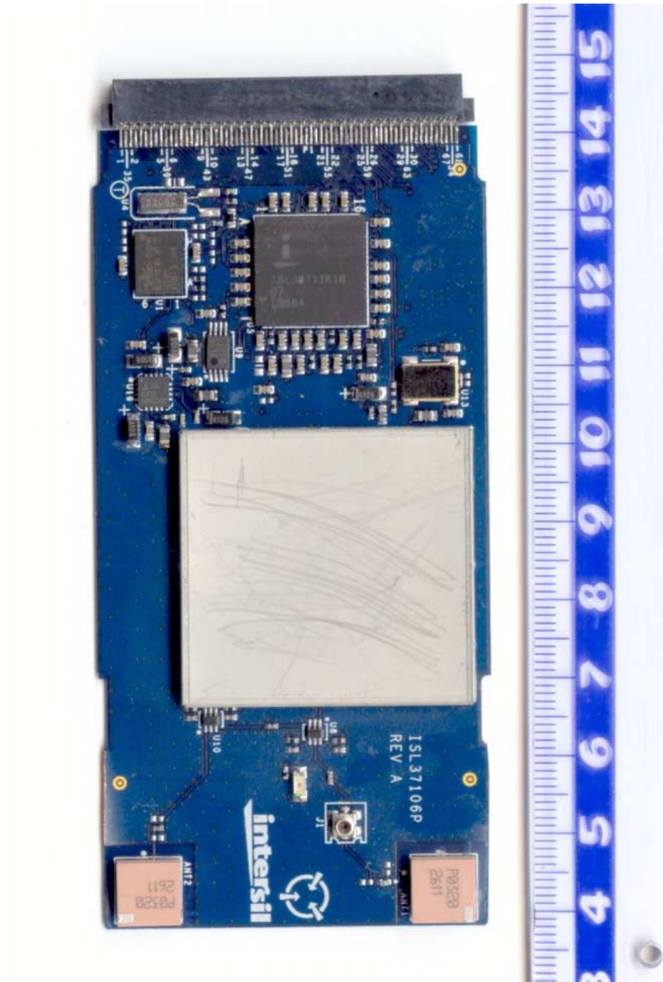
ISL37106P PCB front with shield
