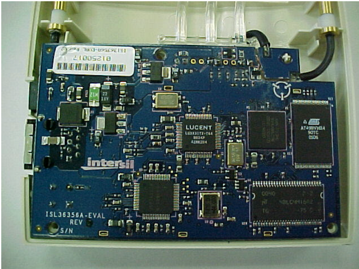
Close-up of PCB.
