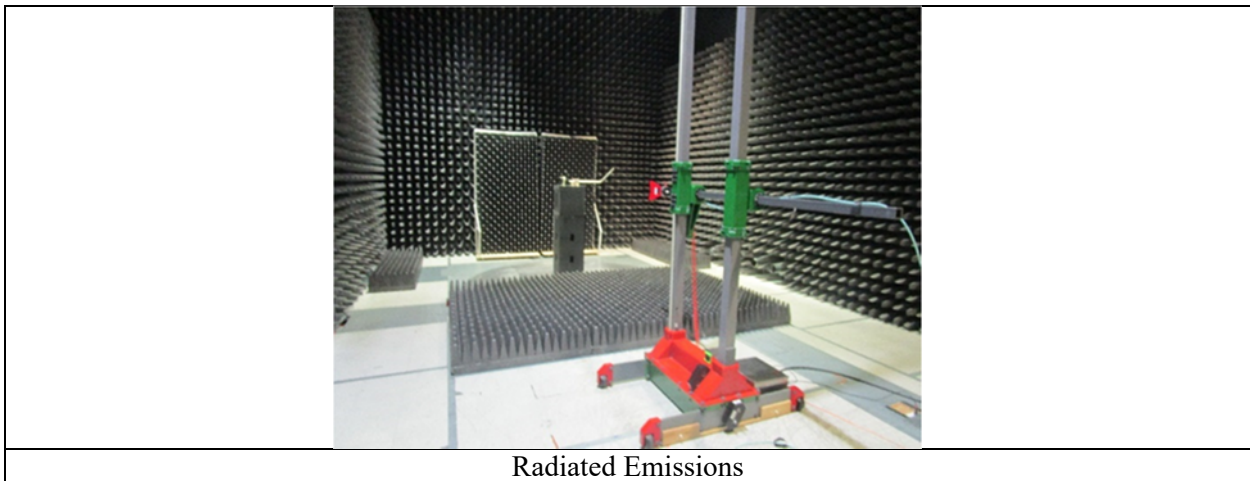
Radiated Emission
