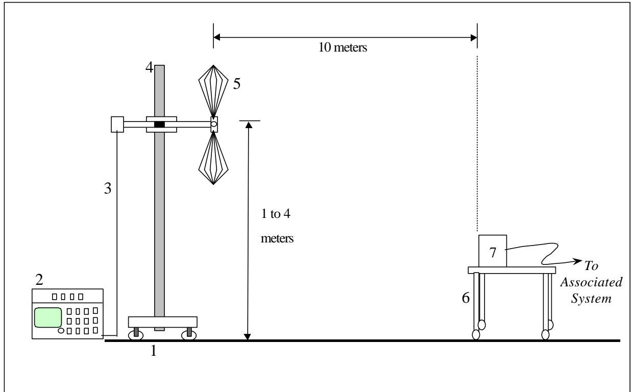
Figure 3. Radiated Emissions Test Setup Drawing
