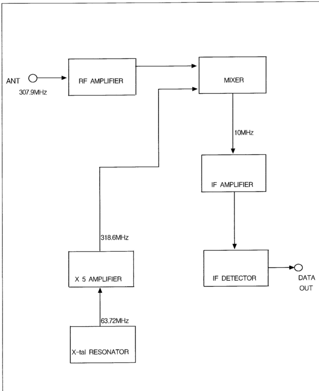
figure 8.1 WMF-R13 Block diagram
