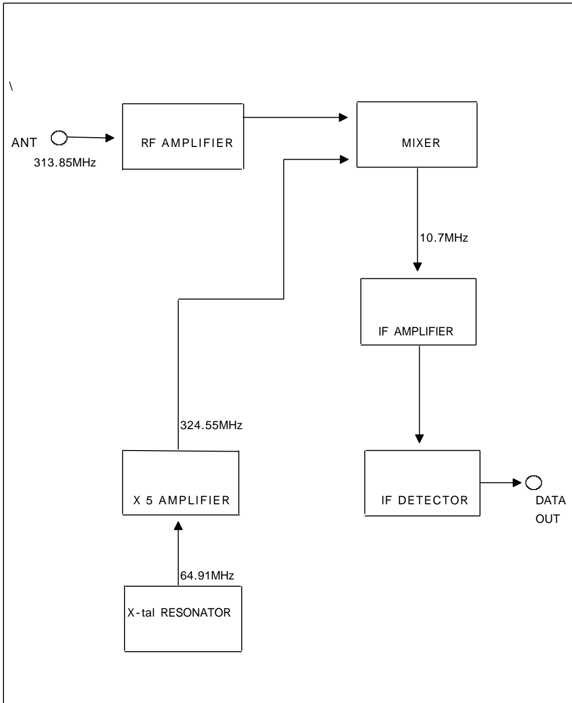
figure 8.1 WMF-R31 Block diagram
