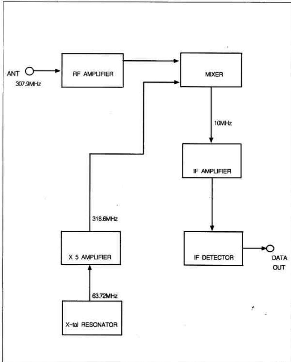
figure 8.1 WMF-R13 Block diagram
