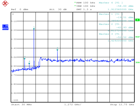
Figure 6. Plot of the Spurious RF conducted emissions
