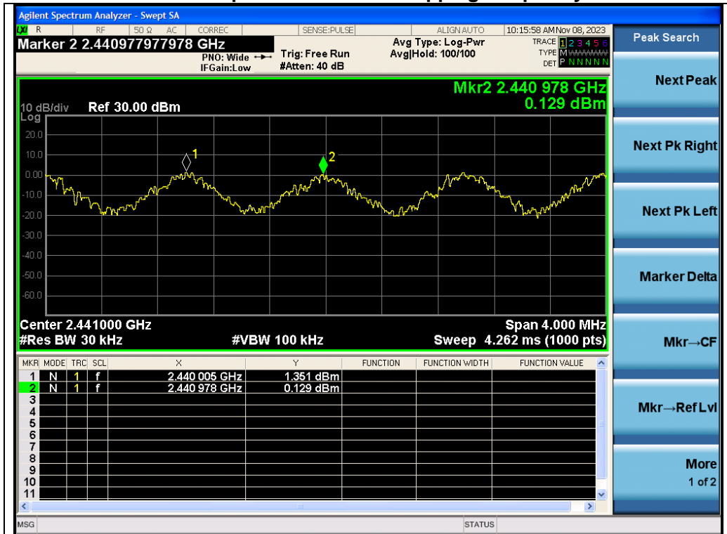
Test_Graph_BR_HOP_ANT1_NA_1Mbps_Hopping Separation
