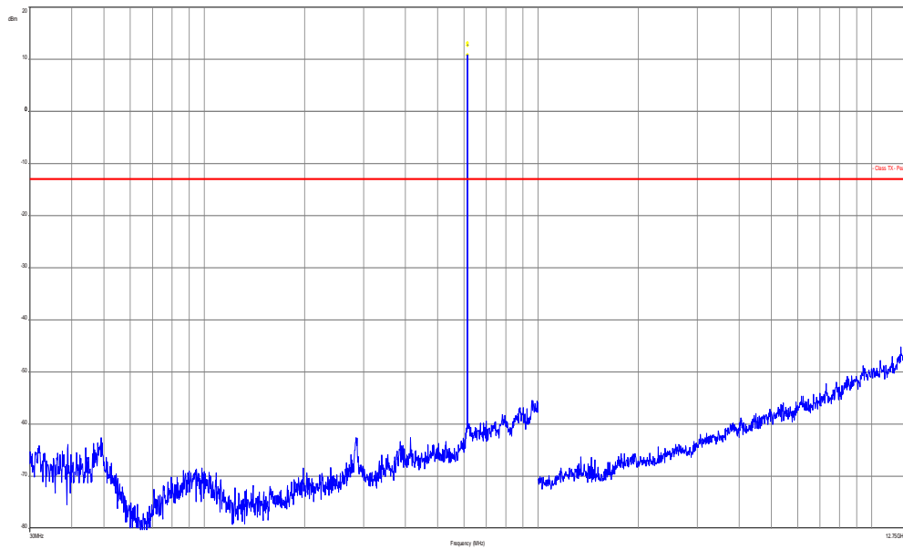
Plot 4: 30 MHz – 12.75 GHz, 614.1 MHz, vertical and horizontal polarisation
