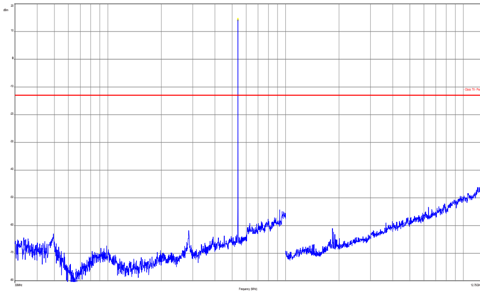
Plot 2: 30 MHz – 12.75 GHz, 539.0 MHz, vertical and horizontal polarisation
