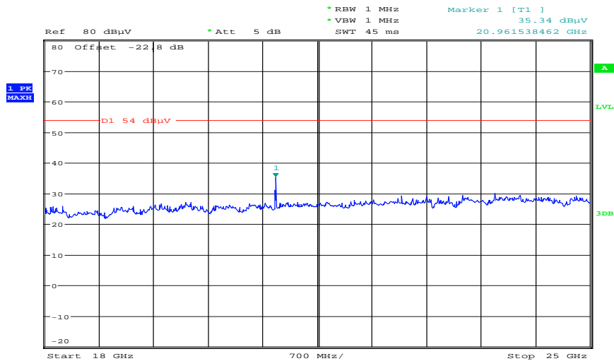
Plot 17: Highest channel, 18 GHz to 25 GHz (vertical / horizontal – max hold – also valid for 20m)
