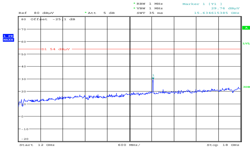
Plot 8: Middle channel, 12 GHz to 18 GHz (vertical / horizontal – max hold – also valid for 20m)
