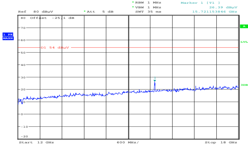
Plot 16: Highest channel, 12 GHz to 18 GHz (vertical / horizontal – max hold – also valid for 20m)
