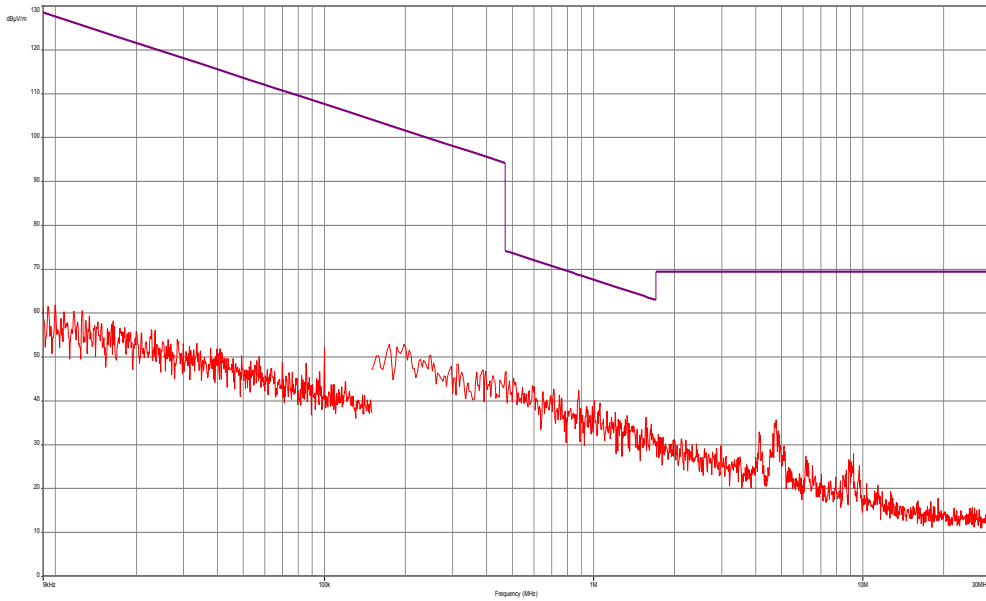
Plot 1: 9 kHz to 30 MHz (Antenna A / B - valid for all channels)
