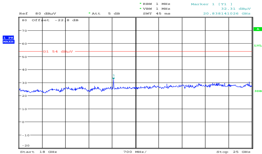
Plot 11: Middle channel, 18 GHz to 25 GHz (vertical / horizontal – max hold – also valid for 20m)
