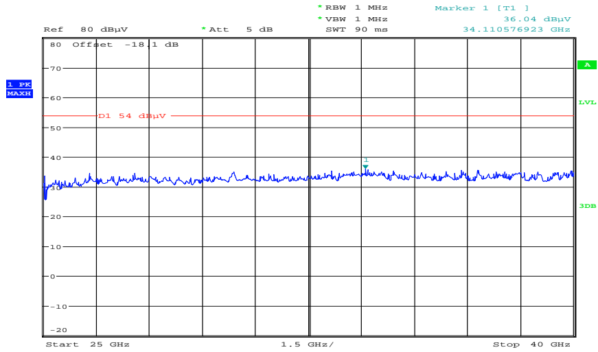
Plot 18: Highest channel, 25 GHz to 40 GHz (vertical / horizontal – max hold – also valid for 20m)
