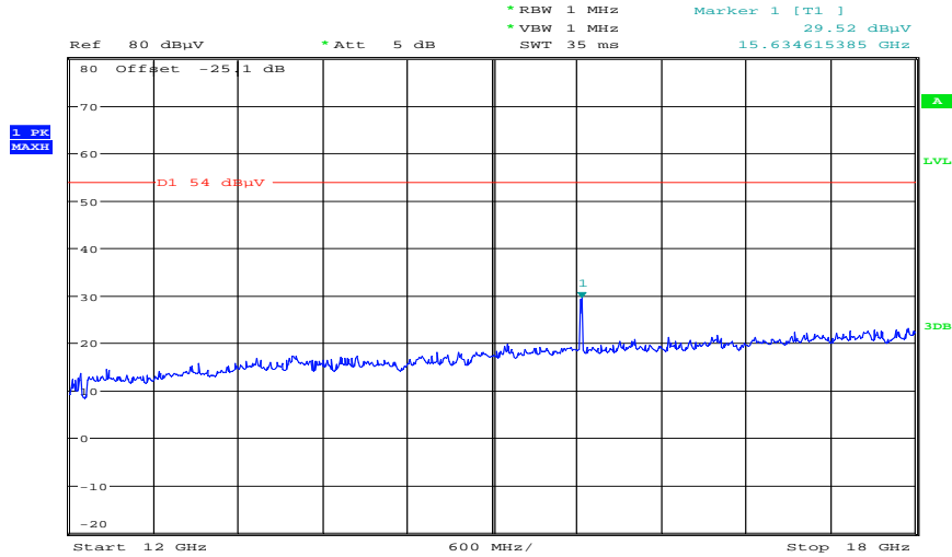
Plot 10: Middle channel, 12 GHz to 18 GHz (vertical / horizontal – max hold – also valid for 20m)
