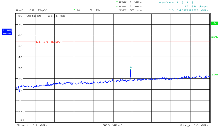
Plot 4: Lowest channel, 12 GHz to 18 GHz (vertical / horizontal – max hold – also valid for 20m)
