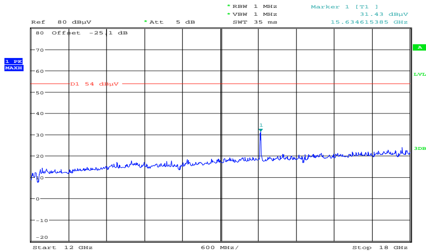
Plot 6: Middle channel, 12 GHz to 18 GHz (vertical / horizontal – max hold – also valid for 20m)
