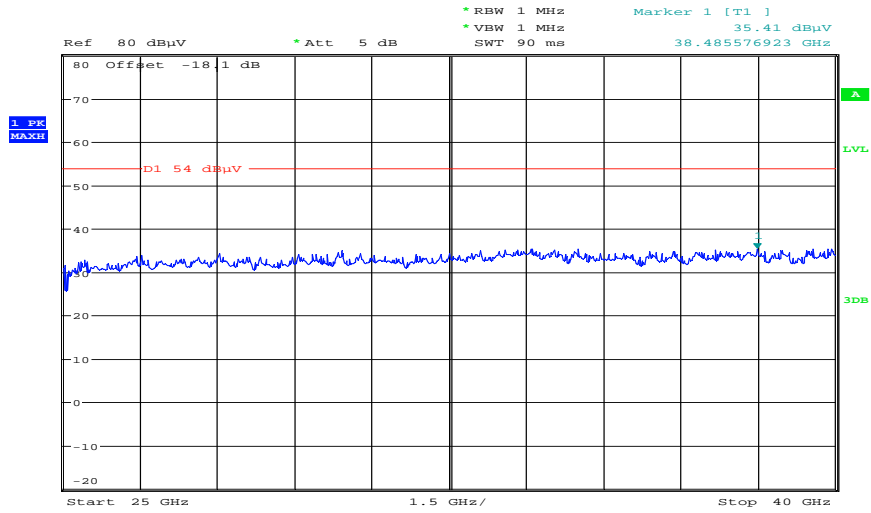
Plot 12: Middle channel, 25 GHz to 40 GHz (vertical / horizontal – max hold – also valid for 20m)
