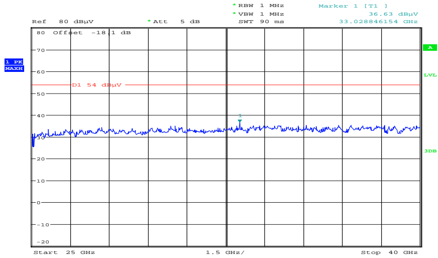
Plot 6: Lowest channel, 25 GHz to 40 GHz (vertical / horizontal – max hold – also valid for 20m)
