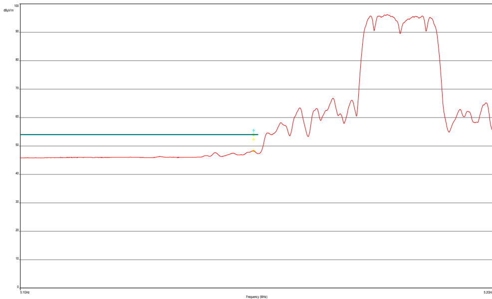
Plot 1: lower band edge, vertical and horizontal polarization
