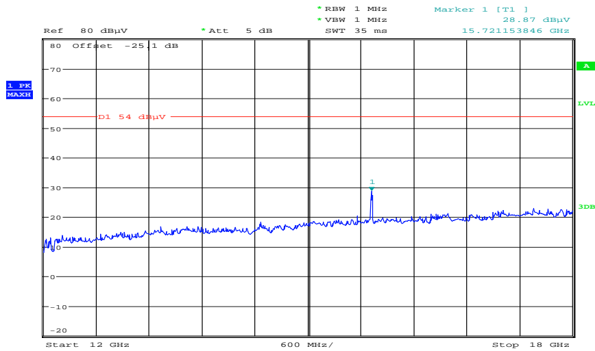
Plot 13: Highest channel, 12 GHz to 18 GHz (vertical / horizontal – max hold – also valid for 20m)
