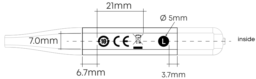
Left aluminum container
