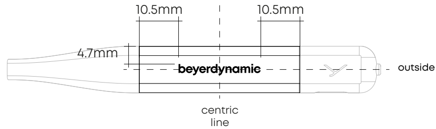
Right aluminum container
