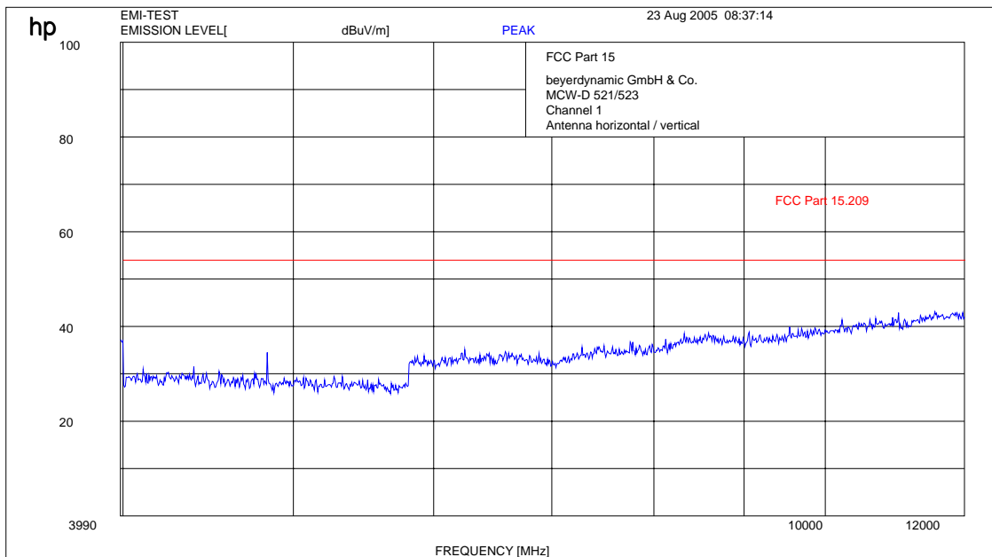
Plot 2: 4- 12 GHz (lowest channel)
